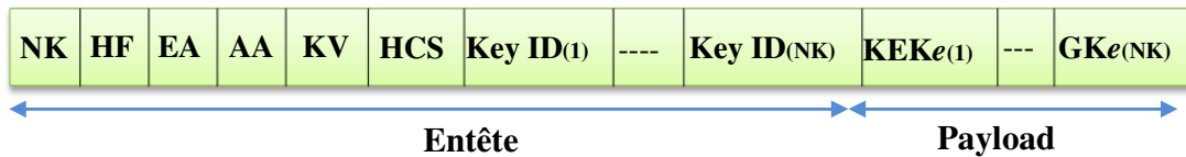
Figure 2.20. Structure de KPDU
