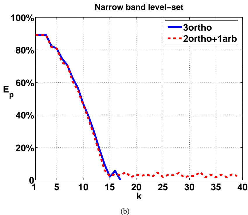
Figure 3.39: Comparison between the '3ortho' and '2ortho+1arb' cases for the sphere reconstruction with the 'Narrow band' method for: (a) the normalized residual r_k with respect to the iteration k ; (b) error in pixels E_p comparing to the original object.
