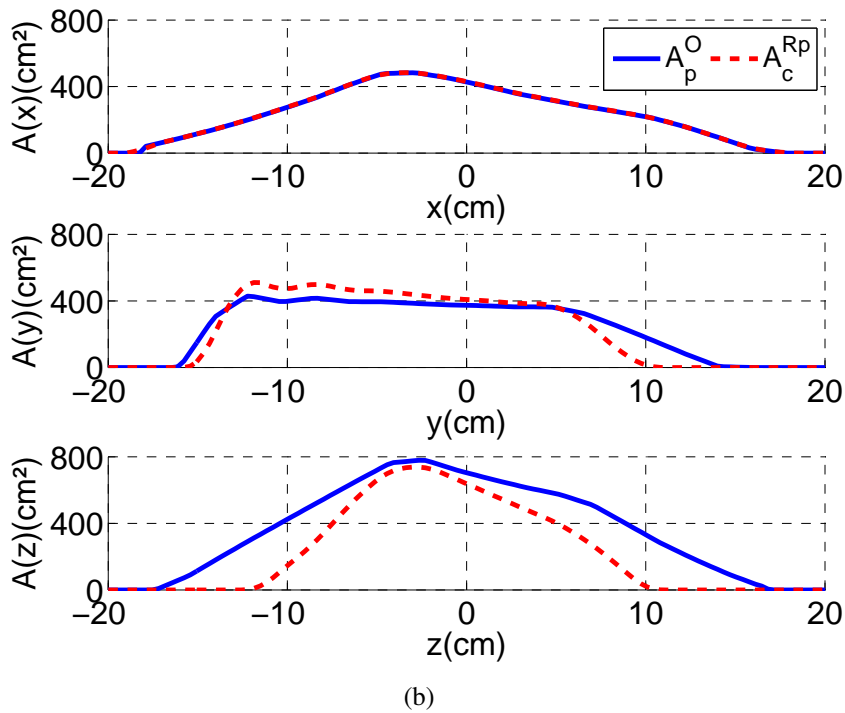
Figure 3.6: Quality evaluation of 3D image reconstruction in Fig. 2.12: (a) Comparison between the analytical geometrical profile functions A_g^O of the initial object and the profile functions A_c^{Rg} computed from its reconstructed object Rg ; (b) Comparison between the physical profile functions A_p^O of the initial object and the profile functions A_c^{Rp} computed from its reconstructed object Rp , in direction x , y , z , respectively.
