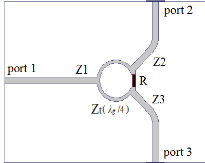
Figure 4.14: Wilkinson divider with stripline
