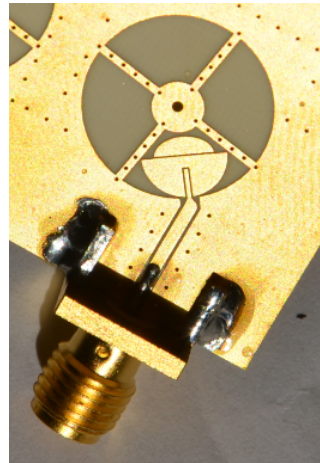
Figure 2.45: Photograph of realized CPW-fed monopole antenna (the other unit on the bottom layer is not presented in this figure).
