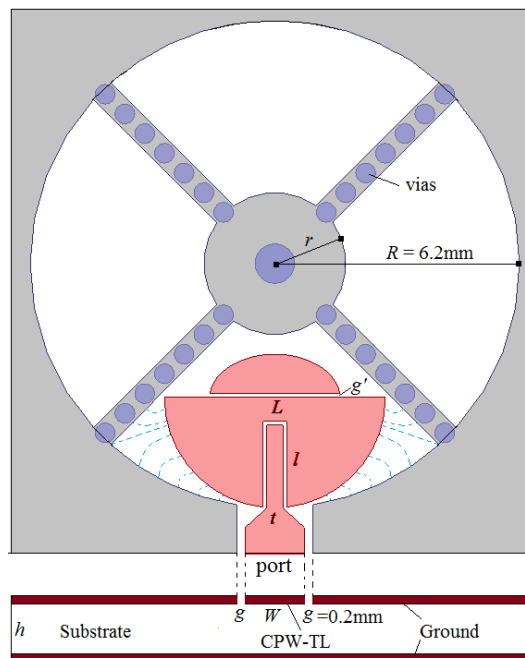
Figure 2.38: Geometry of CPW-fed monopole antenna
