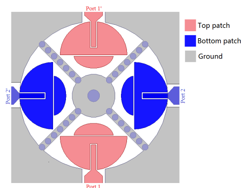
Figure 3.2: Dual-polarized sub-array
