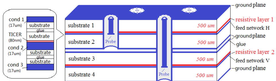
Figure 4.21: Topology of Multilayer PCB technique
