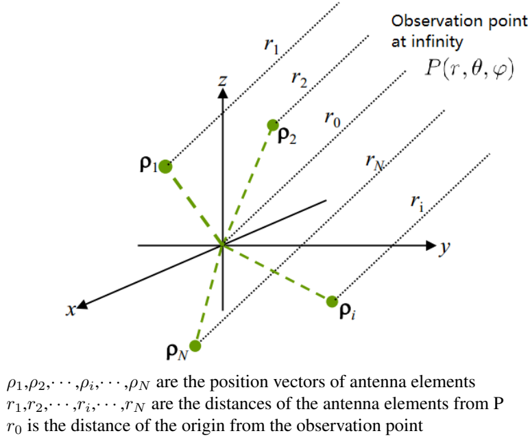
Figure 2.16: Integration of array E-fields.
