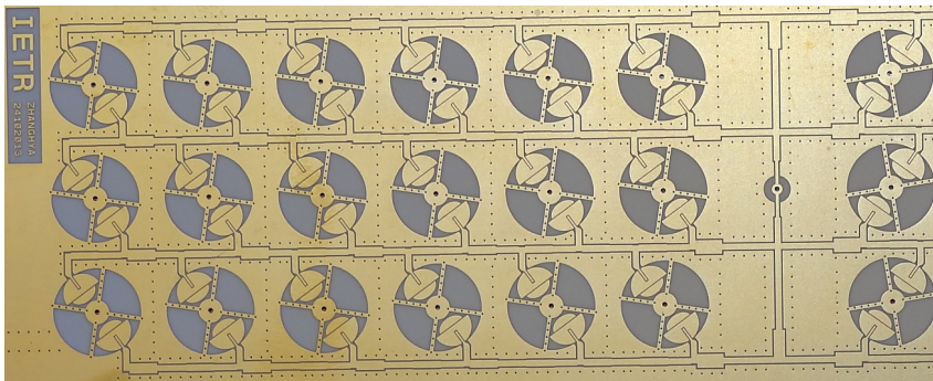
Figure 3.15: Photograph of 3x12 CPW-fed monopole antenna array (part) fabricated in 'PROTECNO GTID' PCB factory of Brest, FRANCE
