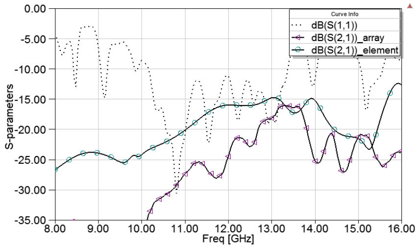
Figure 4.23: Comparison of Isolation between 4x4 array and single element
