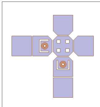
Figure 2.27: Antenna topology when U-slot is used
