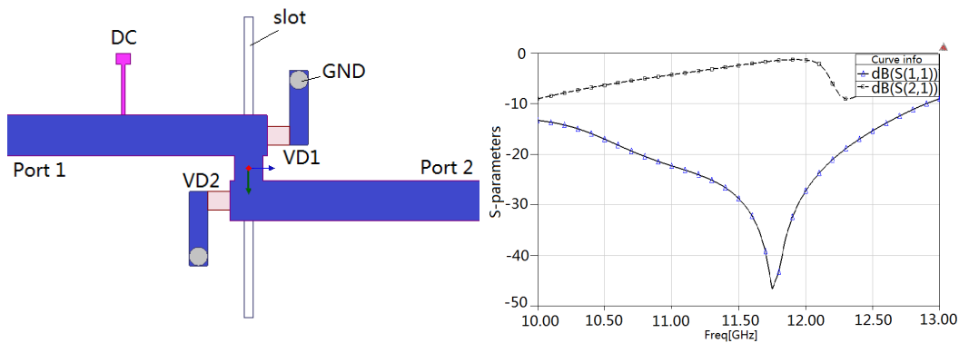
(a)Geometry
