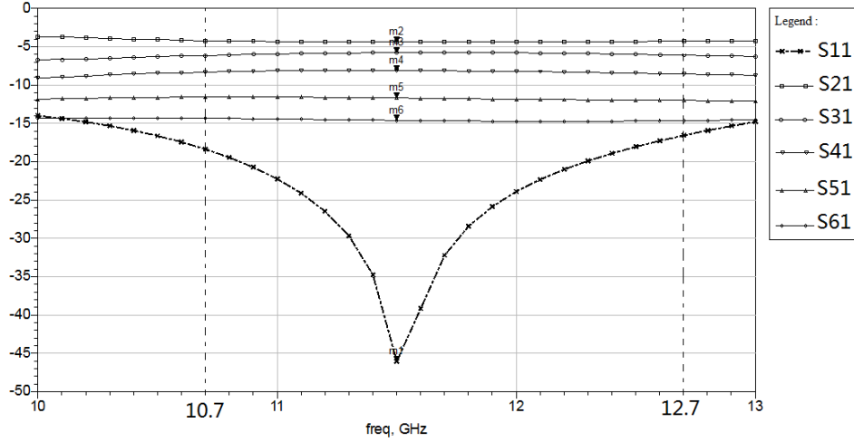
Figure 3.8: Simulated S parameters of feed network
