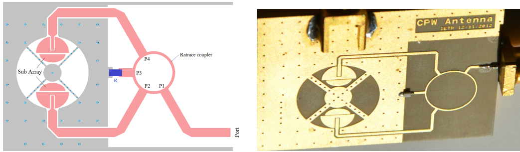
Figure 3.3: Sub-array feed with Ratrace Figure 3.4: Realized sub-array antenna coupler
