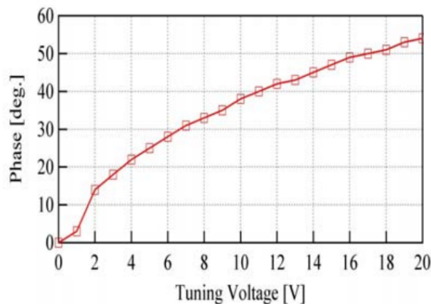
(c)Phase shifting [109]
