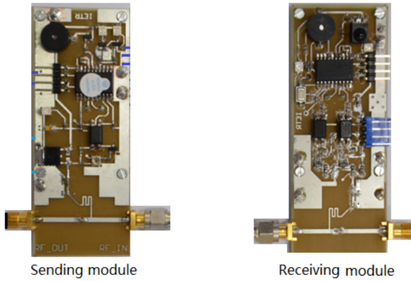
Figure D.3: Realized command transmitting modules
