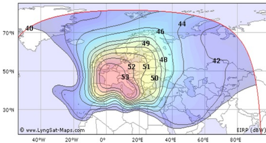
Figure 1.4: EIRP map of hotbird Geo-satellite [4]
