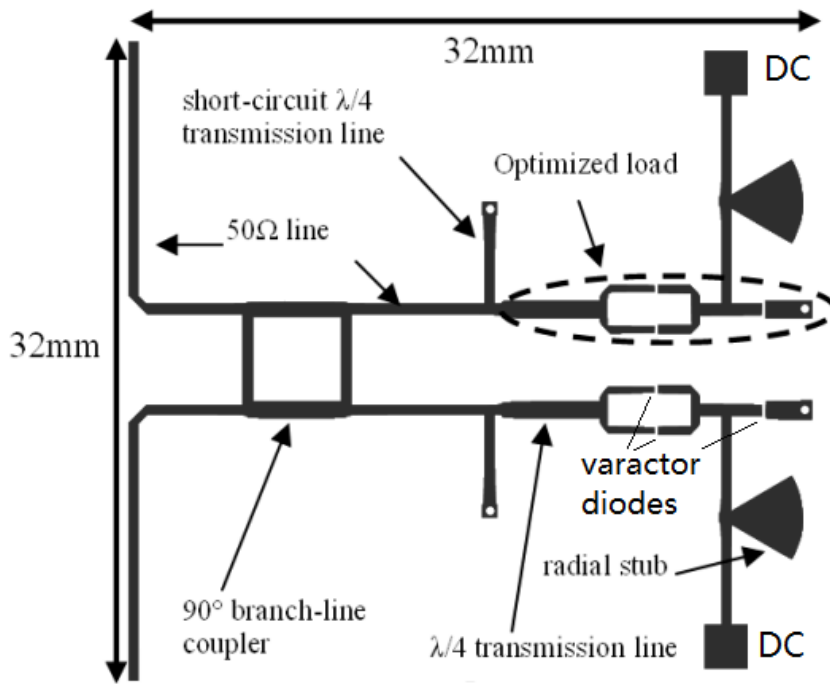
(a)Geometry
