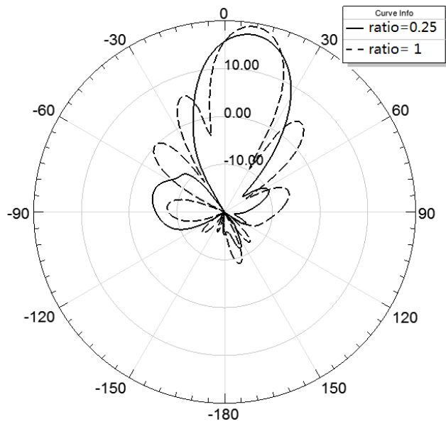
Figure 5.15: Radiation patterns t_{phase} = 41^\circ
