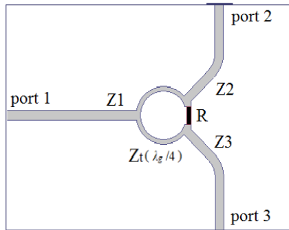
Figure 4.14: Wilkinson divider with stripline Figure 4.15: Comparisons of Wilkinson and T-junction dividers
