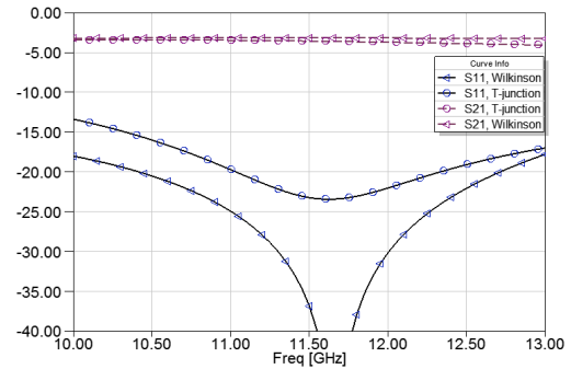
Figure 4.14: Wilkinson divider with stripline Figure 4.15: Comparisons of Wilkinson and T-junction dividers
