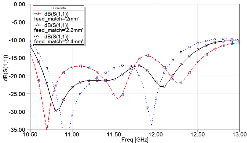
Figure 2.42: Simulated S11 when tuning insert feed length
