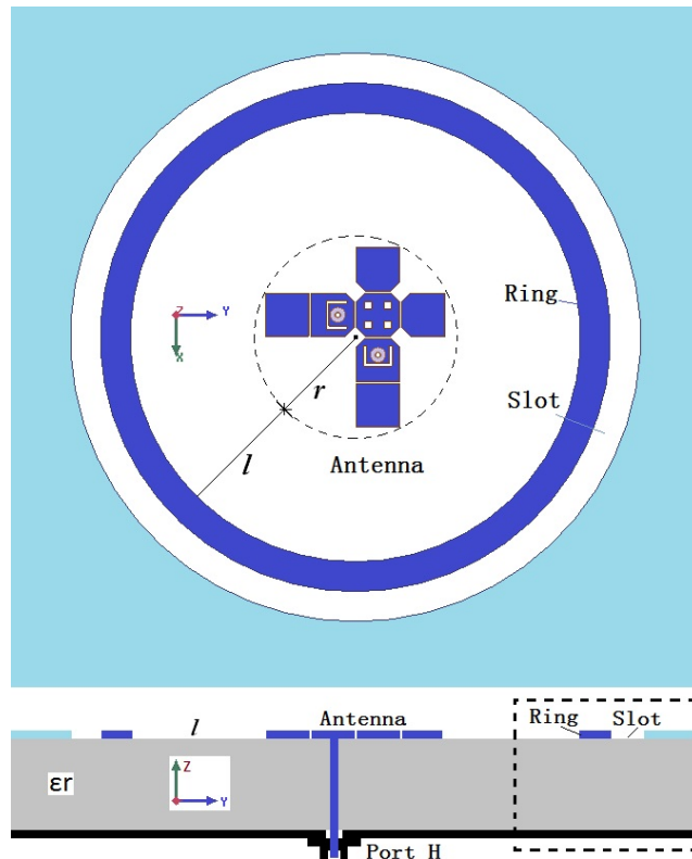
Figure 2.36: Cross-type antenna with sidelobe suppression structure
