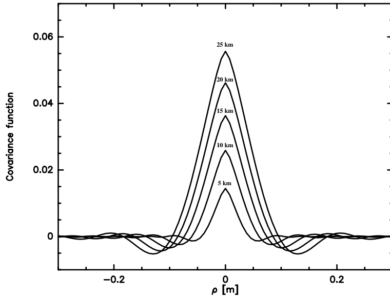
Figure I.2: Covariance function C_1(\rho) of irradiance due to a single turbulent layer, with optical turbulence factor J = 3 \cdot 10^{-14} [\text{m}^{1/3}] , at different distances: h = 5, 10, 15, 20, 25 km. The wavelength is \lambda = 0.53 \mu\text{m} .
