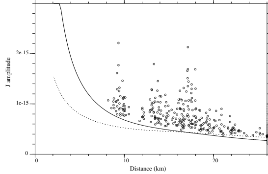
Figure I.6: \tilde{J} amplitude of the components (small circles) detected with the CLEAN algorithm along the different observing sequences. The sensitivity threshold of our SCIDAR observations is shown as a solid curve. The dashed curve is the noise floor as given by (Eq. I.14) for the TBL ( D=2 m plus central obscuration). Observations with PISCO in 1998: \gamma Ari with \sigma_I^2=0.14 , N_{ph}=110 photons and d_0=17 km
