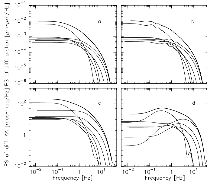
Figure I.10: a-b) Power spectrum of differential piston (interferometer) and c-d) Power spectrum of differential Angle-of-Arrival (mono-pupil) for each one of the turbulence layers, and for their summation (thick lines). a) and c) is along the star separation, and b) and d) is perpendicular to that direction, that is mainly along the wind direction. The outer scale of turbulence is 50 m. The star separation angle is 2' with single dish observations.
