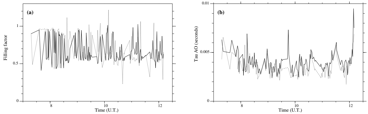
Figure II.6: Filling factor (a), and \tau_{AO} (coherence time for full correction Adaptive Optics) (b) obtained with automatic (solid line) and interactive (dashed line) procedures, versus the time of observation (night of 19/05/2000).
