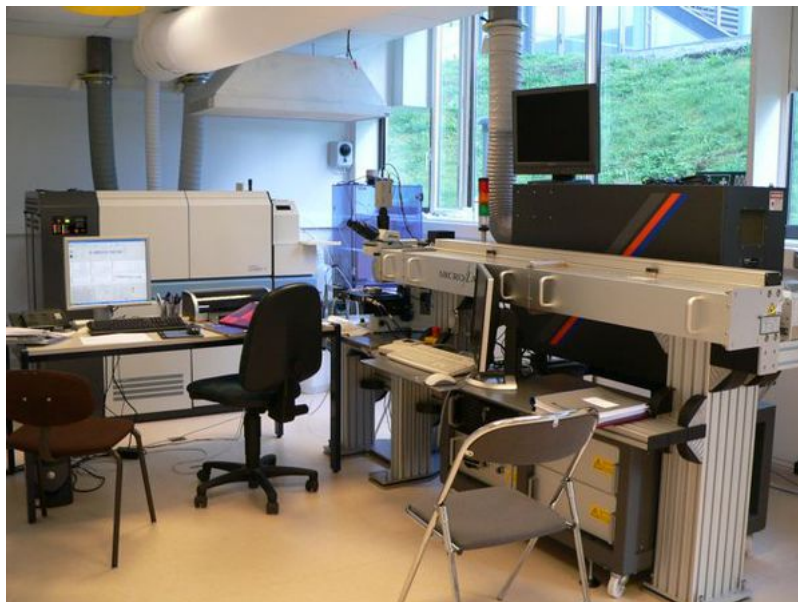
FIGURE 3.3 – Photo de l'HR-ICP-MS Thermo Element II (+ LASER) du PSO (IUEM)
