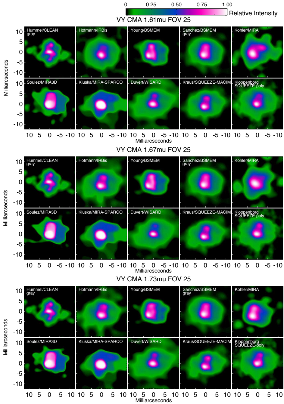
Figure 5. This panel shows all the images from the contestants for VY CMA, in each of the three narrow spectral bands. East is left, North is up and the field-of-view is 25x25 milliarcseconds. The images are scaled by the peak surface brightness. The color table is non-linear and a color bar gives a more quantitative feeling for the surfaces brightness levels for each entry. The effective angular resolution varied between the entries and no attempt was made to convolve entries to a common angular resolution (see text for more detail).
