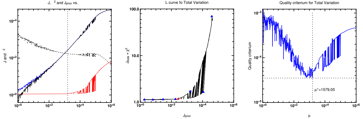
Fig. B.1. Tuning the hyper-parameter \mu for the total-variation regularization with MiRA/SPARCO. Left : cost functions vs. the hyper-parameter \mu . Red line: \chi^2 ( =\mathcal{J}_{\text{data}} ). Black dashed line: 1000 \times \mathcal{J}_{\text{prior}} (multiplied by 1000 for better graph visibility). Black solid line: \mu \mathcal{J}_{\text{prior}} . Blue line: \mathcal{J} = \mu \mathcal{J}_{\text{prior}} + \chi^2 . The vertical dotted line corresponds to the best regularization weight \mu^+ found by the quality criterium. Center : The L curve is one of the criteria to choose the regularization weight \mu . Black line: the values of \mathcal{J}_{\text{data}} vs. \mathcal{J}_{\text{prior}} for a range of \mu values from 1 to 10^6 . Blue triangles: points where \mu = \{1, 10, 10^2, 10^3, 10^4, 10^5, 10^6\} . Red triangle: the value where \mu = \mu^+ . Right : the quality criterium graph is the distance between the pixels of the reconstructed image to the real (here the model) one. Blue line: the value of the quality criterium vs. the hyper-parameter \mu . Dotted line: the position of the minimum of the curve and the corresponding value of \mu = \mu^+ .
