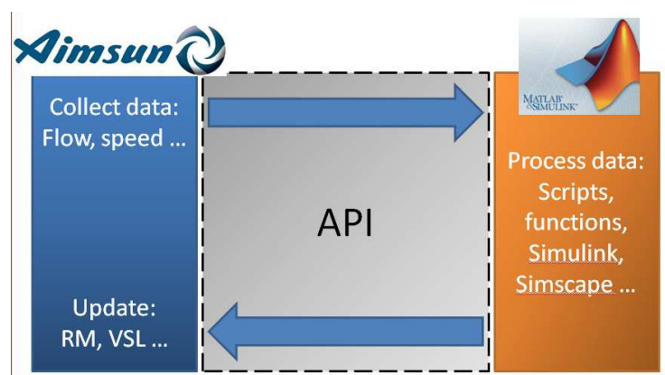
Figure 7.5: API developed to provide communication between Matlab and Aimsun.
