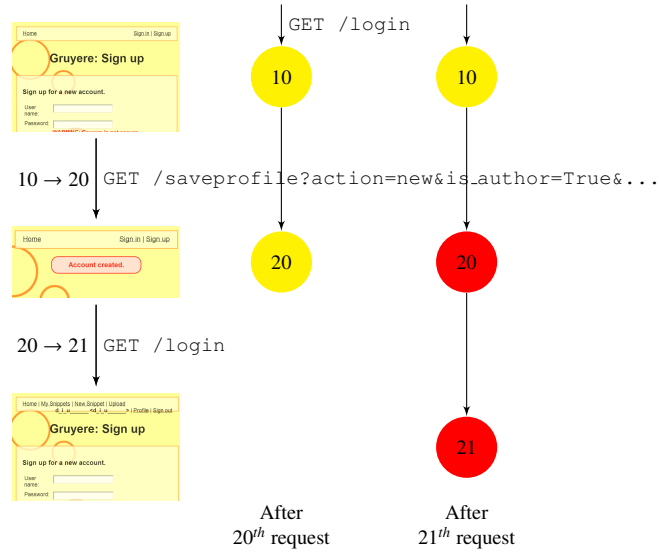
Figure 4.3: Evolution of the Navigation Tree when the Macro-State Changes
