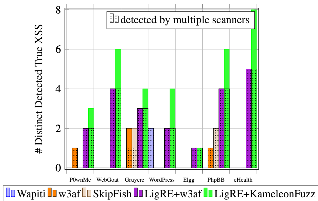
Figure 6.4: Detection Capabilities of Black-Box XSS Scanners
