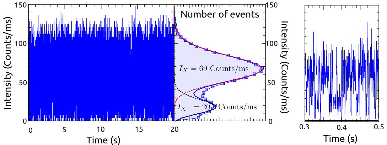
Figure III.6 – Example of a typical timetrace for DR3.2 at \langle N_{\text{eh}} \rangle = 0.3 . Left: Photoluminescence for a 20 s duration, bin time \Delta t = 250 \mu\text{s} . The corresponding histogram is shown (middle). Two states are clearly visible, a fit with two Poisson distributions (blue line) reproduces well the measured histogram and gives I_X = 69 \text{ Counts/ms} and I_{X^-} = 20 \text{ Counts/ms} . Right: zoom on a 200 ms time window, the maximum duration of the two states appears to be of the order of 10 ms.
