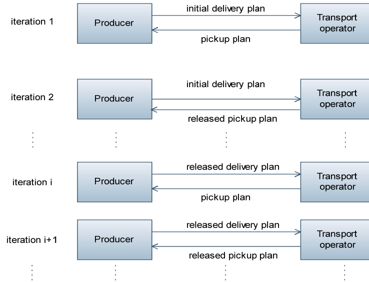
Figure 3.10 Negotiation iterations
