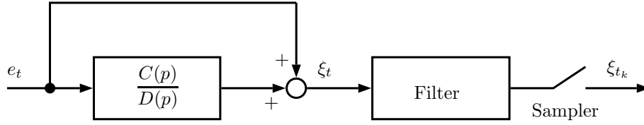
Figure 2.3: The block diagram of the integrated sampling scheme.
