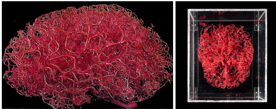
Figure 1.19: A so-called “corrosion cast” of the blood vessels in the brain. The level of details required to image this structure in 3D in vivo is beyond the capabilities of current imaging devices.
