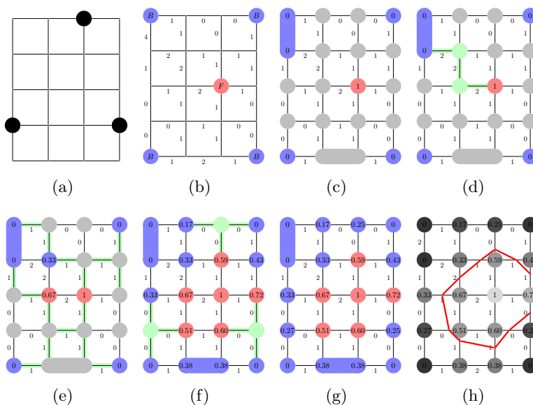
Figure 4.13: (a) Three dots in a 4 \times 5 lattice. (b) Associated lattice weighted by an Euclidean distance map from the dots, with Foreground and Background seeds. (c) First steps of the power watershed algorithm optimizing (4.31) in the case q = 2 and p \rightarrow \infty . Nodes with a maximum weight are merged. (d) A plateau of weight 2 (in green) including different seeded nodes is encountered. The Random walker algorithm is applied to label the nodes on the plateau. (e,f) New plateaus of weight 1 and 0 are encountered, the Random walker algorithm is applied, (g) Final labeling x solution of (4.31). The resulting isocontour is represented in red.
