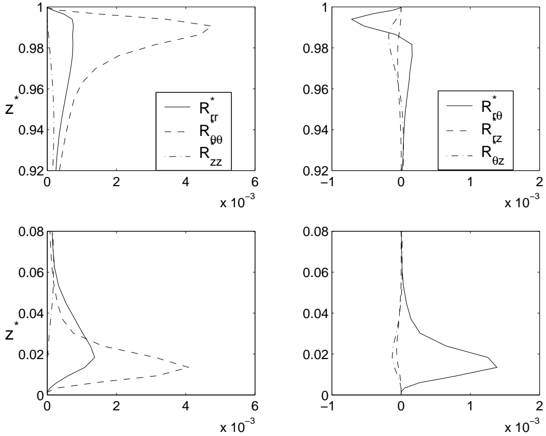
Figure 8.11: Axial variations of the Reynolds stress tensor components in the stator (top graphs) and rotor (bottom graphs) boundary layers for r^* = 0.5 , G = 1/7 , R_m = 1.8 and Re = 10^6 using the LES-SVV.
