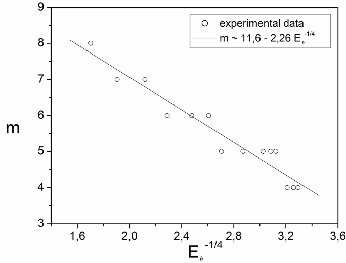
Figure 6.11: Evolution of the number of vortices with the Ekman number based on the water depth at rest for \eta = 0 and increasing values of Re . Results obtained by flow visualizations.
