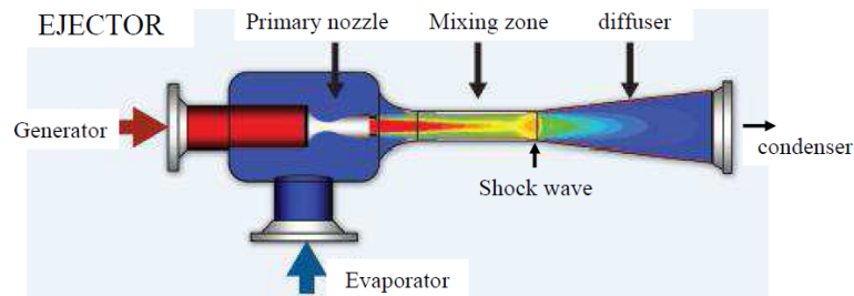
Figure 14.6: Operating principle of an ejector (CanmetEnergie).
