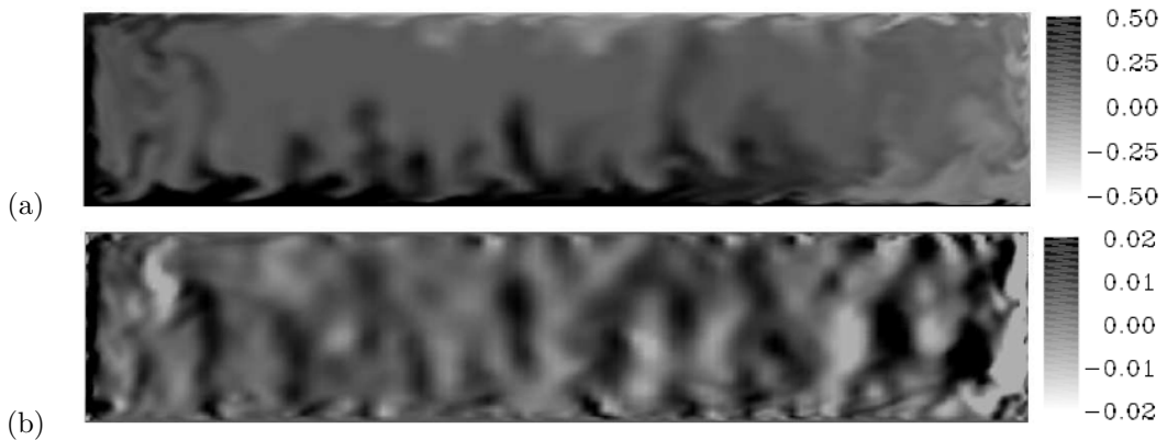
Figure 8.22: Iso-values of (a) the instantaneous temperature T^* and (b) the instantaneous axial velocity V_z normalized by \Omega b in a (r, z) plane. Results obtained using the LES-SVV for G = 1/7 , R_m = 1.8 , Re = 10^6 and Ra = 10^7 .
