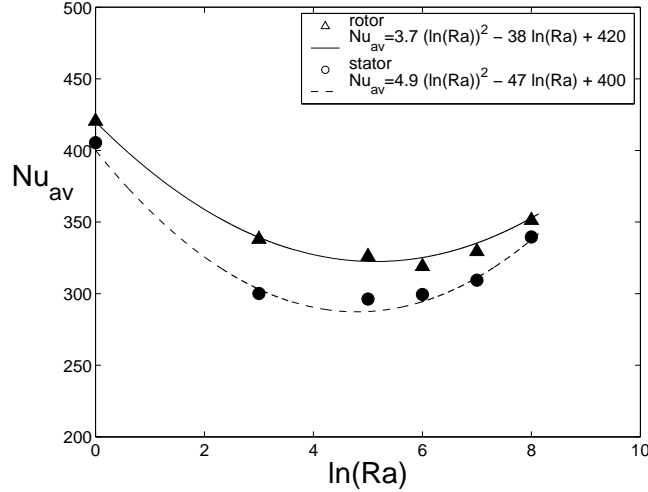
Figure 8.31: Influence of the Rayleigh number Ra on the averaged Nusselt number Nu_{av} on both disks. Results obtained using the LES-SVV for G = 1/7 , R_m = 1.8 and Re = 10^6 .
