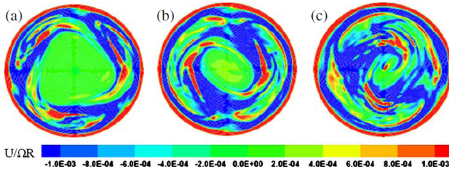
Figure 8.37: Unsteady vortical structures obtained by the three-dimensional k - \varepsilon modeling of Craft et al. [60] for \Omega = 724 rpm and G = 0.195 near the stator. Contours of axial velocity after: (a) 20 disk revolutions, (b) 40 revolutions, (c) 70 revolutions.
