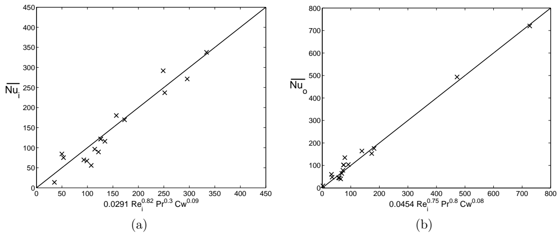
Figure 12.14: Correlations for the averaged Nusselt numbers along the: (a) inner cylinder and (b) the outer cylinder for all the considered cases. Results obtained by the in-house RSM for \Gamma = 77 and \eta = 0.961 .
