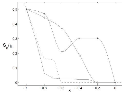
Figure 9.9: Size S_c/h of the smallest cell against s for G = 1.8 (RSM). Comparison between (—) the smooth disk case ( Re = 1.3 \times 10^6 ), (---) the bladed disk case ( Re = 2 \times 10^5 ) and previous numerical results of (*) Kilic et al. [154] and (◇) Gan et al. [102] in the smooth disk case.
