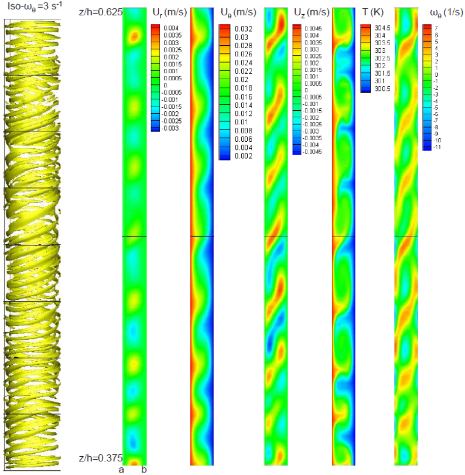
Figure 10.10: WSPI regime ( Ta = 75 , Ra = 7150 ). From left to right: iso-values of the azimuthal vorticity \omega_\theta and maps of the three velocity components, the temperature and the azimuthal vorticity in a ( r \in [a, b] , z/h \in [0.375, 0.625] ) plane.
