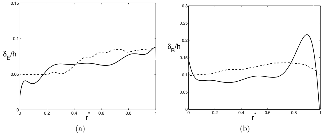
Figure 8.14: Radial distributions of the boundary layer thicknesses: (a) Ekman boundary layer thickness \delta_E/h , (b) Bödewadt boundary layer thickness \delta_B/h . Comparisons between (—) the present LES-SVV ( Re = 10^6 , G = 1/7 , R_m = 1.8 ) and (---) the predictions of the Reynolds Stress Model of Poncet [249] ( Re = 1.04 \times 10^6 , G = 0.036 , R_m = 1.36 ).
