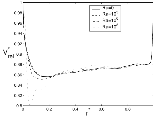
Figure 8.30: Radial distributions of the relative velocity V_{rel}^* along the rotor ( z^* = 0.99 ) for four values of the Rayleigh number. Results obtained using the LES-SVV for G = 1/7 , R_m = 1.8 and Re = 10^6 .
