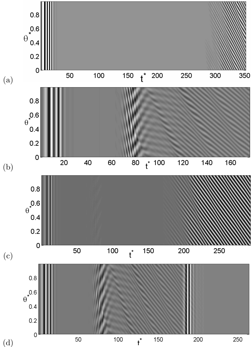
Figure 7.7: Space-time diagrams of the axial velocity V_z^* = V_z/(\Omega r) deduced from the DNS for Re = 24630 , G = 0.114 and R_m = 1.8 . \theta^* = \theta/(2\pi) is the azimuthal angle on a fixed circle at r^* = 0.604 and z^* = 0.812 . (a) Case 1, (b) Case 2, (c) Case 3, (d) Case 4.
