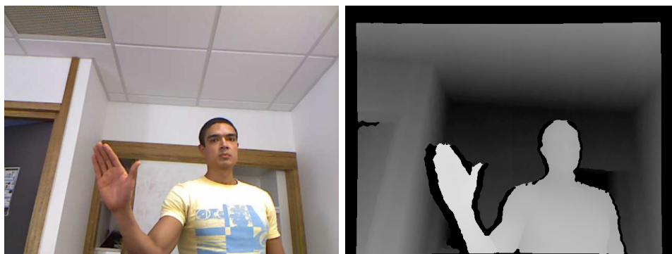
Fig. 2.1: RGBD representation. (a) RGB image and (b) depth image. The depth image is encoded in gray levels, where the closer a point is at the brighter is drawn. Pixels having no valid depth measures are drawn in black. Note that field of views of RGB and depth cameras are different.
