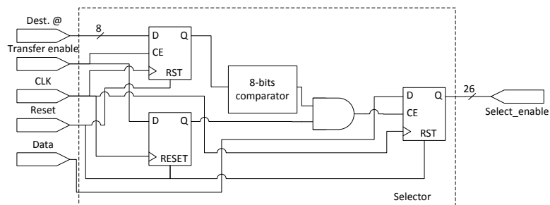
Figure 3.10: Selector architecture overview
