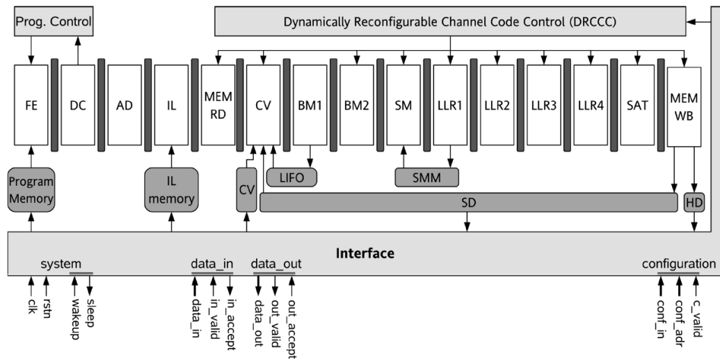
Figure 1.14: FlexiTreP general architecture
