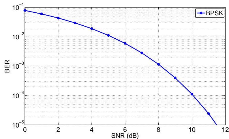
FIGURE 1.12 – BER vs SNR
