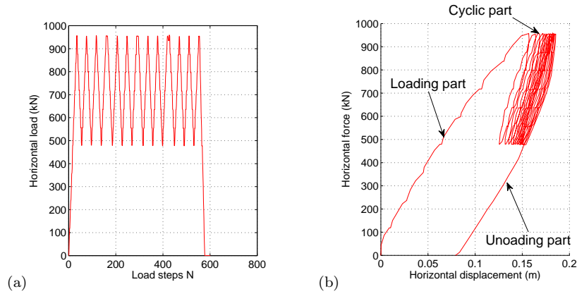
Figure 6.21: Experimental data (from Rosqu et [1]) used to calibrate the hypoplastic macro-element: (a) loading; (b) pile head response
