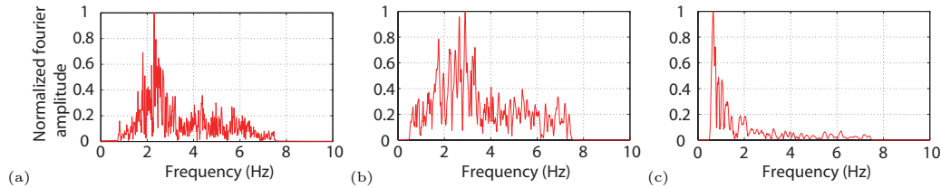
Figure 4.2: Frequency representations of the base shaking: (a) Martiniqne Jara, (b) Northridge earthquake and (c) Kobe earthquake
