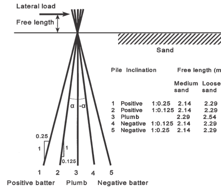
Figure 2.28: Layout of single battered pile for static centrifuge tests, Zhang et al. [12]
