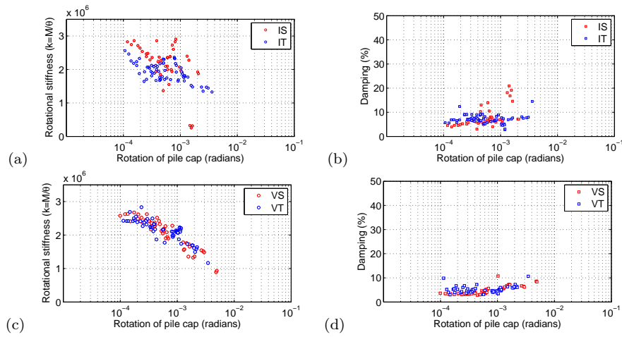
Figure 4.58: Rotational stiffness degradation curves, real earthquake input: Inclined pile group with (a) short and tall building and (b) damping ratio; (c) Vertical pile group with short and tall building and (d) damping ratio
