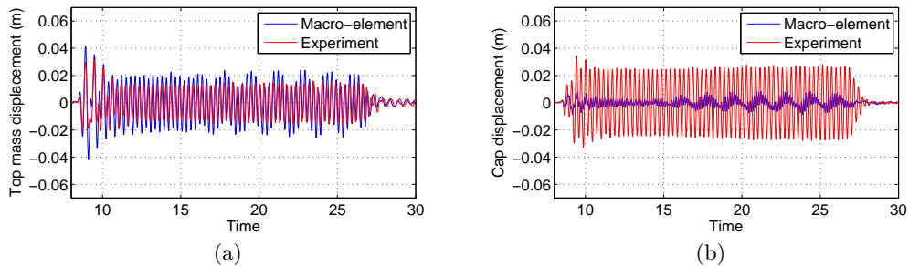
Figure 6.38: Validation of macro-element for vertical pile group: vertical pile group with short building under sine 3.5 Hz 0.4 g input: (a) response of top mass; (b) response of pile cap
