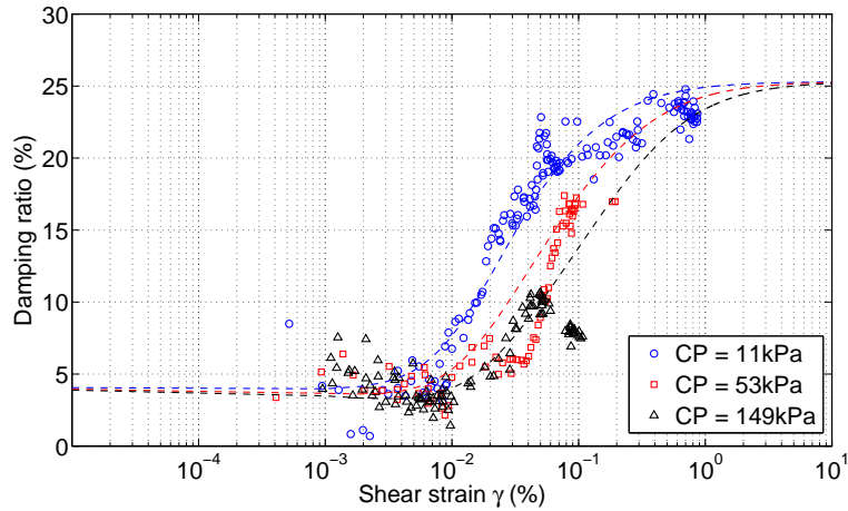
Figure 3.22: Influence of the confining pressure (CP) on the evolution of the damping ratio of the Fontainebleau sand. Experimental data Vs. empirical equation results
