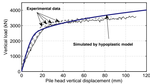
Figure 5.17: Hypoplastic model with intergranular strain: Numerical Vs. experimental results for a single pile submitted to vertical compression
