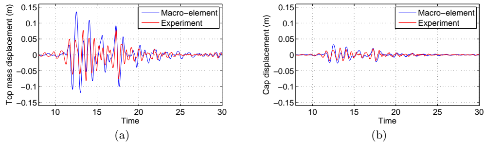
Figure 6.40: Validation of macro-element for vertical pile group: vertical pile group with tall building under Kobe -4 dB earthquake: (a) response of top mass; (b) response of pile cap
