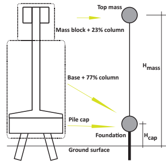
Figure 4.7: Foundation-superstructure discretization
