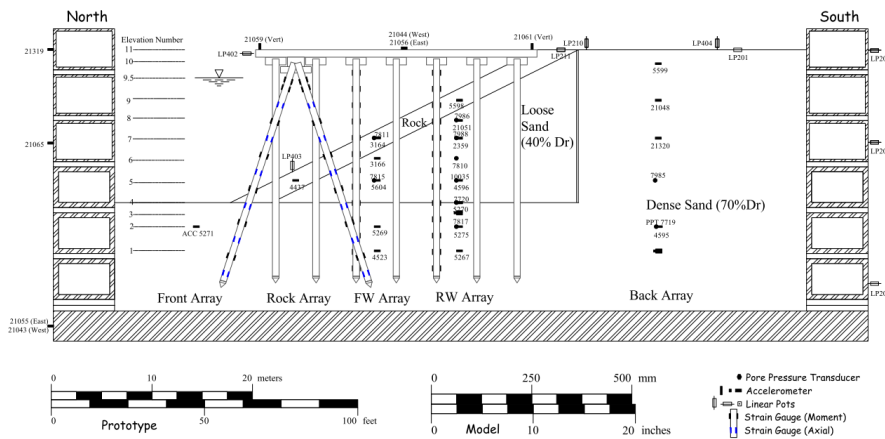
Figure 2.34: Center cross Sections of the centrifuge models, instruments locations for the JCB01 model, Boland et al. [17]
