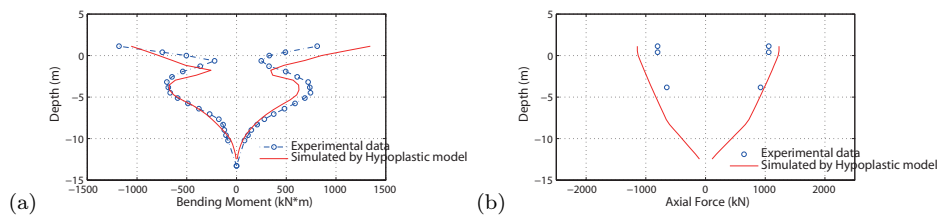
Figure 5.19: Comparison of numerical results of vertical pile group with short superstructure, real earthquake excitation (Northridge -9 dB): (a) Bending moment and (b) axial force
