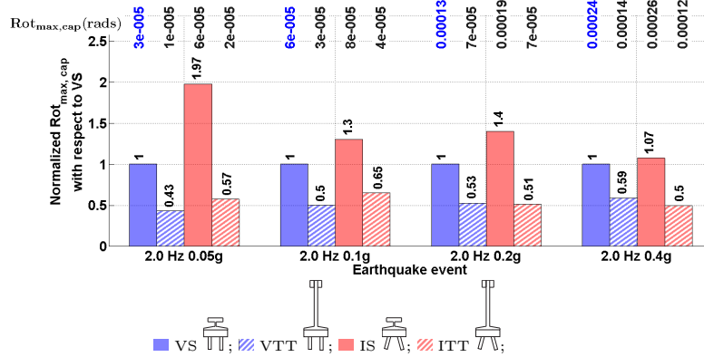
Figure 4.39: Normalized maximum rotation of pile cap, under 2.0 Hz sinusoidal excitations
