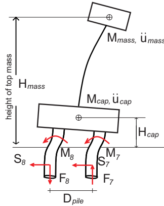
Figure 4.20: Illustration of the movements of pile cap and forces acting on the foundation system
