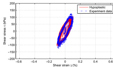
(b) Depth 14.4m, confining pressure 128 kPa
