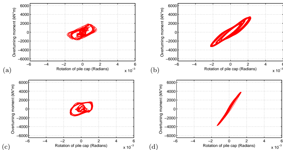
Figure E.2: Rotation-moment Hysteresis loops, 3.5 Hz sine input: (a) Inclined pile group with short building; (b) Vertical pile group with short building; (c) Inclined pile group with tall building (14.16 m) and (d) Vertical pile group with tall building (14.16 m)
