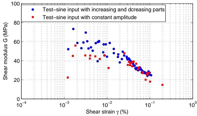
Figure 3.15: Dynamic centrifuge tests: Shear modulus Vs. shear strain of the Fontainebleau sand layer at depth 5.4m (confining pressure 53kPa) – two types of loading signal
