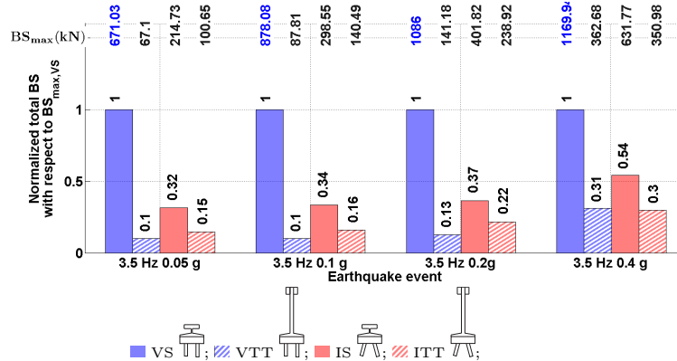
Figure 4.42: Normalized maximum base shear, under 3.5 Hz sinusoidal excitations
