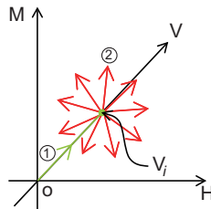
Figure 6.6: Radial displacements in the H - M plane at the vertical load level V_i
