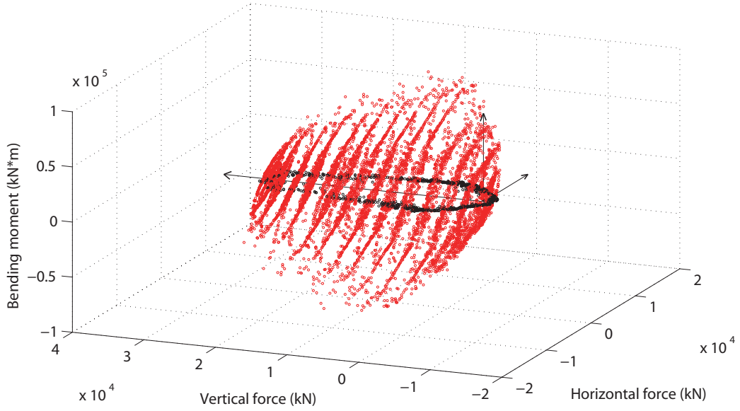
Figure 6.9: Numerical failure envelope in the H-M-V space
