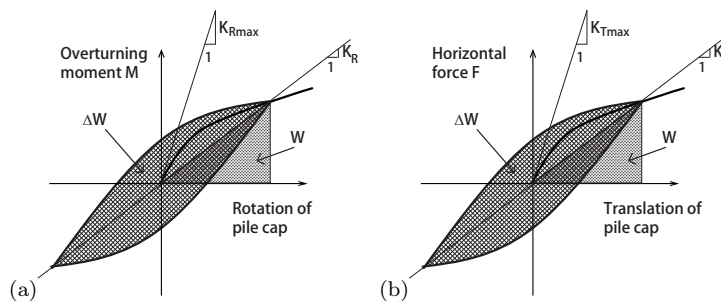
Figure 4.23: Illustration of calculation of equivalent rotational, translational stiffness and associated damping ratio: (a) rotational stiffness and damping ratio; (b) translational stiffness and damping ratio
