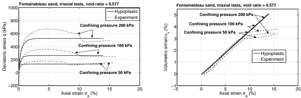
Figure 5.10: Triaxial compression tests on dense Fontainebleau sand, void ratio = 0.577, simulation vs. experiments
