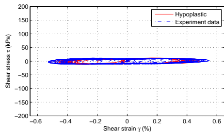
(a) Depth 1.2m, confining pressure 21 kPa
