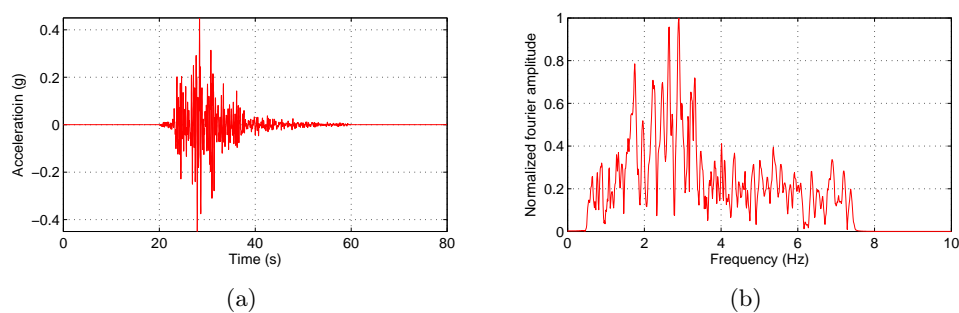
Figure A.20: Time (a) and frequency (b) representation of Northridge -9 dB earthquake
