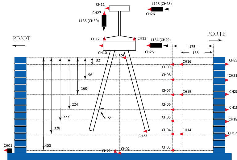
Figure A.8: Sensors planning – inclined pile group with tall building, real earthquake
