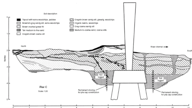
Figure 2.17: Pier C, trench log. (after Berrill et al. [8])
