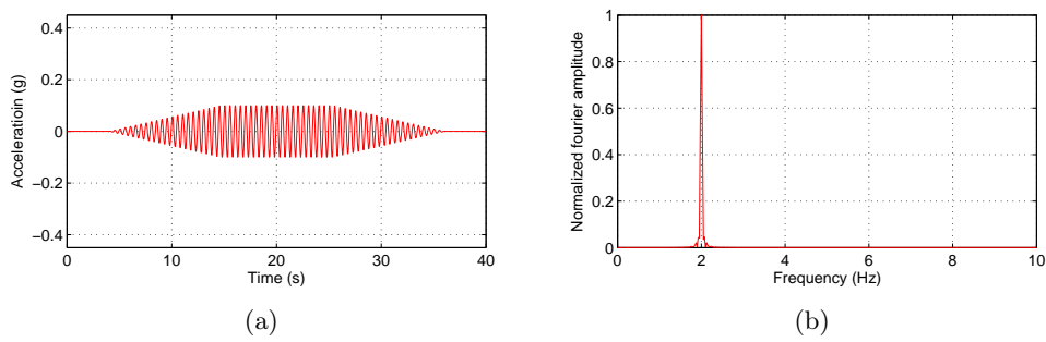
Figure A.31: Time (a) and frequency (b) representation of sine input 2.0 Hz 4g with tapered parts
