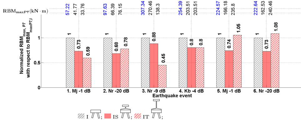
Figure D.8: Normalized maximum residual bending moment, under real earthquake excitations
