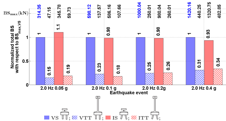
Figure 4.41: Normalized maximum base shear force, under 2.0 Hz sinusoidal excitations
