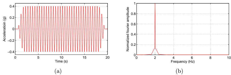
Figure A.25: Time (a) and frequency (b) representation of sine input 80 Hz 16g earthquake
