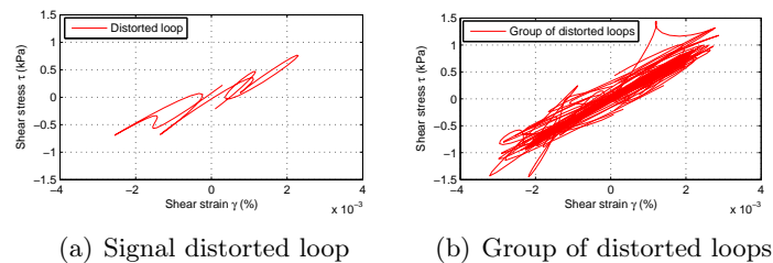
Figure 3.10: Dynamic centrifuge tests: Distorted hysteresis loop (a) and group of distorted hysteresis loops (b)
