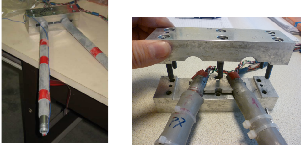
(a) Assembly of inclined piles and pile cap
