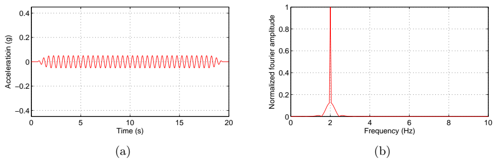
Figure A.22: Time (a) and frequency (b) representation of sine input 2.0 Hz 2g earthquake
