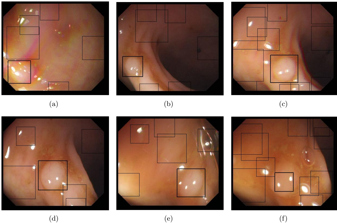
Figure 2.17: Detection examples
