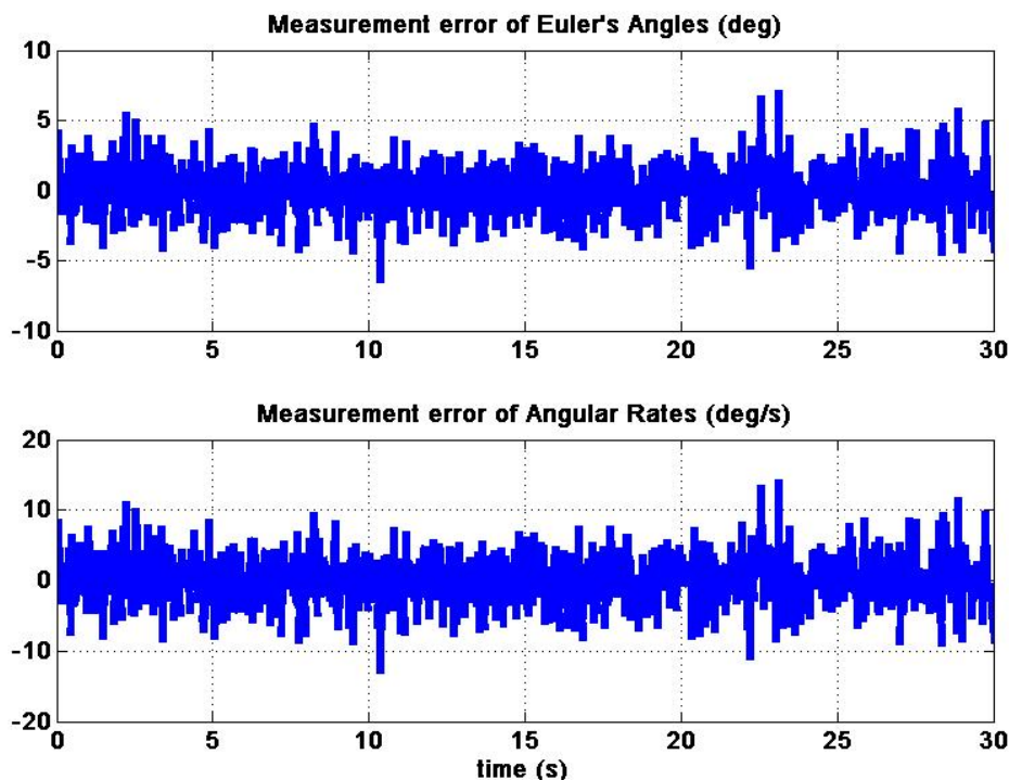
Figure 2.7: Measurement errors of the state variables
