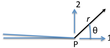
Figure 1.3: Rectangular co-ordinate system at the crack tip P.
