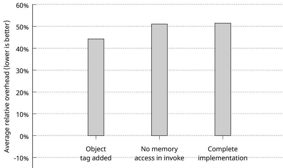
Figure 4.9: Execution overhead of the small objects micro-benchmark when run on partial implementations of the monitoring subsystem, compared to the “Zero implementation”. Overhead is an average of 10 runs.
