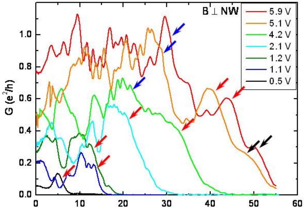
Figure 5.23: Magnetoconductance for different applied gate voltages in the perpendicular magnetic field at T = 4.2 K, sample A. Conductance drops corresponding to the loss of conducting channels marked by the arrows.
