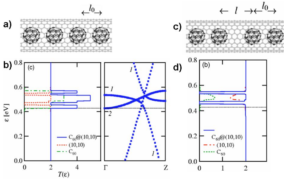
Figure 4.9: a) Model of the periodic C_{60}@ (10,10) peapod, l_0 = 0.9845 nm. b) The transmission (left) and the band structure (right) of periodic C_{60}@ (10,10) around Fermi energy. c) Model of the nonperiodic C_{60}@ (10,10) peapod. d) The transmission of nonperiodic C_{60}@ (10,10) ( l = 1.2036 nm) around Fermi energy. Dashed and dashed-dotted lines show contributions to the transmission from (10,10) nanotube and C_{60} , respectively. Dotted lines show Fermi energy. [Kondo 2005]
