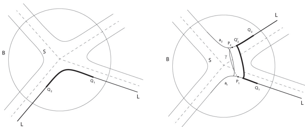
Figure 6.2: Making L contained in \partial S in \mathcal{N}(\mathcal{D}^0) : easy case at the left and general case at right. The dotted lines are 1-simplexes in \mathcal{D}^1 , while the bold segments from Q_1 to Q_2 represent the push-offs of L in \mathcal{N}(\mathcal{D}^0) .
