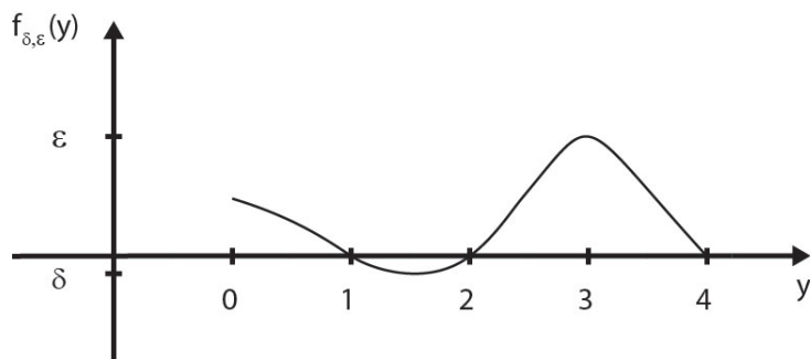
Figure 7.1: The function f_{\delta, \epsilon} on [0, 4] .
