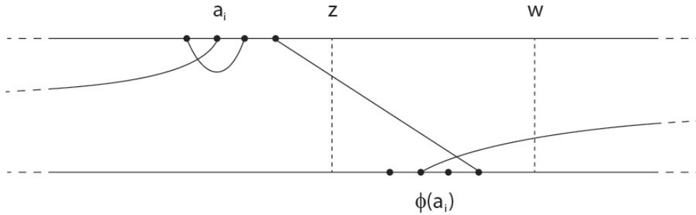
Figure 7.6: Examples of curves \mathfrak{c}_i \in \mathfrak{C}(u) projected on [0, 1] \times K' . Note the curve crossing [0, 1] \times \{w\} can not exist if n_w(u) = 0 .
