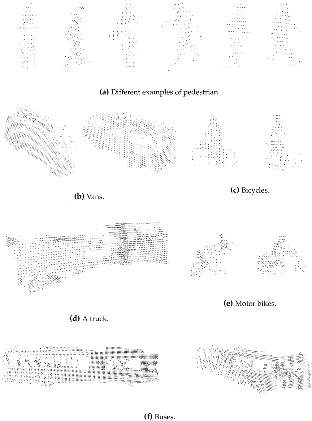
Figure 4.17: Some examples of the hand-labeled data used for training different classifiers.
