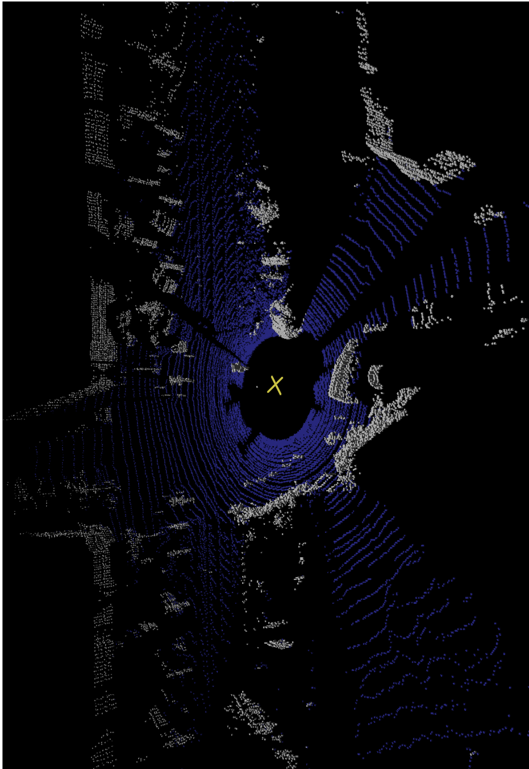
Figure 4.3: Ground segmentation results for a single scan in an outdoor scenario with a grid resolution of 0.1m. Ground voxels are displayed in blue and other occupied voxels in grey. The '+' symbol represents the position of the laser scanner.
