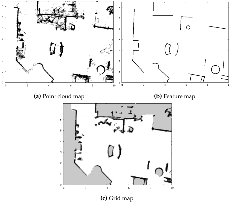
Figure 2.3: Example of different map representations built from the same set of range measurements acquired from a 2D laser scanner.
