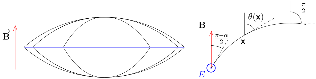
FIGURE 1. A lens \Omega : the magnetic field is nowhere tangent to the boundary and it makes the angle \theta(\mathbf{x}) with the regular boundary.
