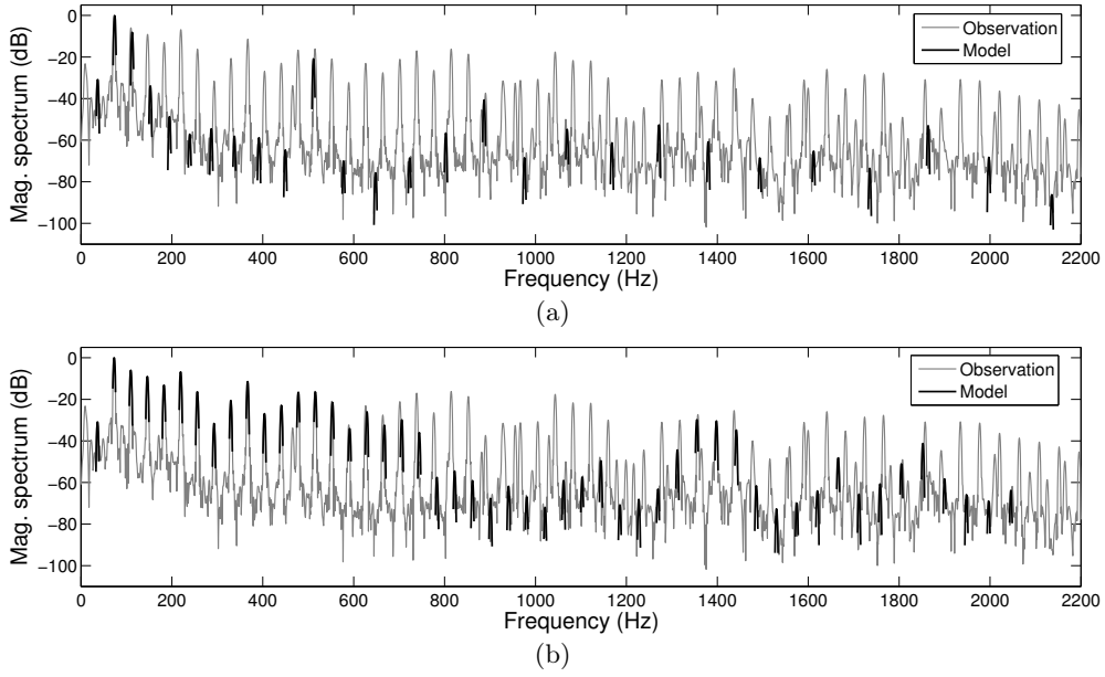
Figure 3.1: Initialization of the NMF models for the analysis of a note D1 . (a) Rough initialization with F_0 set to Equal Temperament and B = 5 \cdot 10^{-3} . (b) Initialization using the model of inharmonicity and tuning along the whole compass of pianos.
