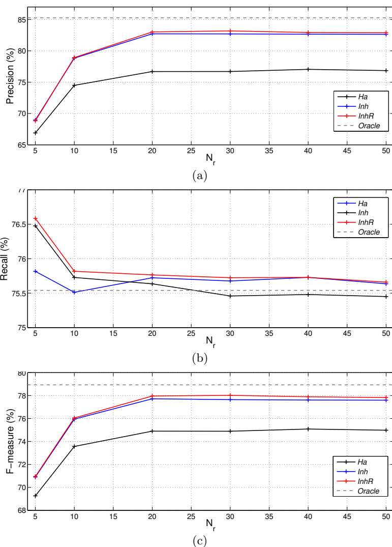
Figure 5.6: (a) Precision, (b) Recall and (c) F-measure (in %) obtained for all methods as a function of the number of partials N_r for T_{\text{on}} = -22 dB.
