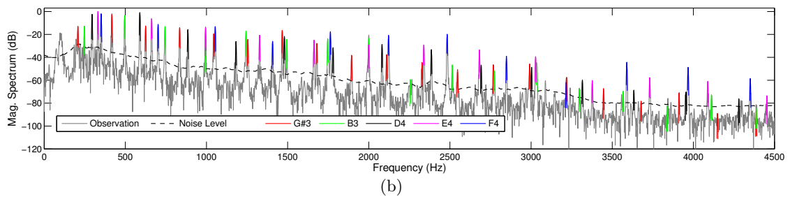
Figure 3.17: Result of InhR-NMF for the analysis of (a) the chord #2 (G \flat 1-A1-C2-E2-G2) and (b) the chord #3 (G \sharp 3-B3-D4-E4-F4) of MAPS SptkBGCl piano.
