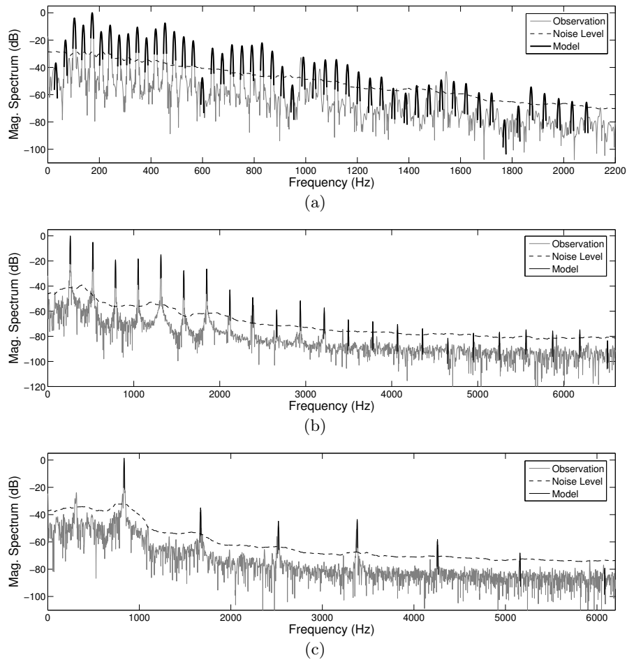
Figure 3.8: Results of InhR-NMF for the analysis of notes (a) C#1, (b) C4 and (c) G#5 of Iowa grand piano.
