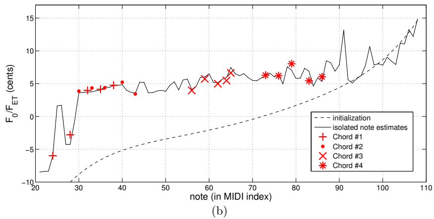
Figure 3.16: InhR-NMF isolated note vs. chord analysis for the MAPS SptkBGCl grand piano. (a) Inharmonicity coefficient and (b) F_0 as dev. from ET along the compass.
