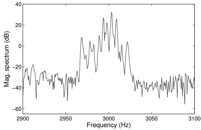
Figure 2.11: Zoom along the frequency axis of the spectrum of a note G b 6 composed of a triplet of strings. Multiple peaks are present while the simple model of transverse vibration for a single string assumes a single partial.
