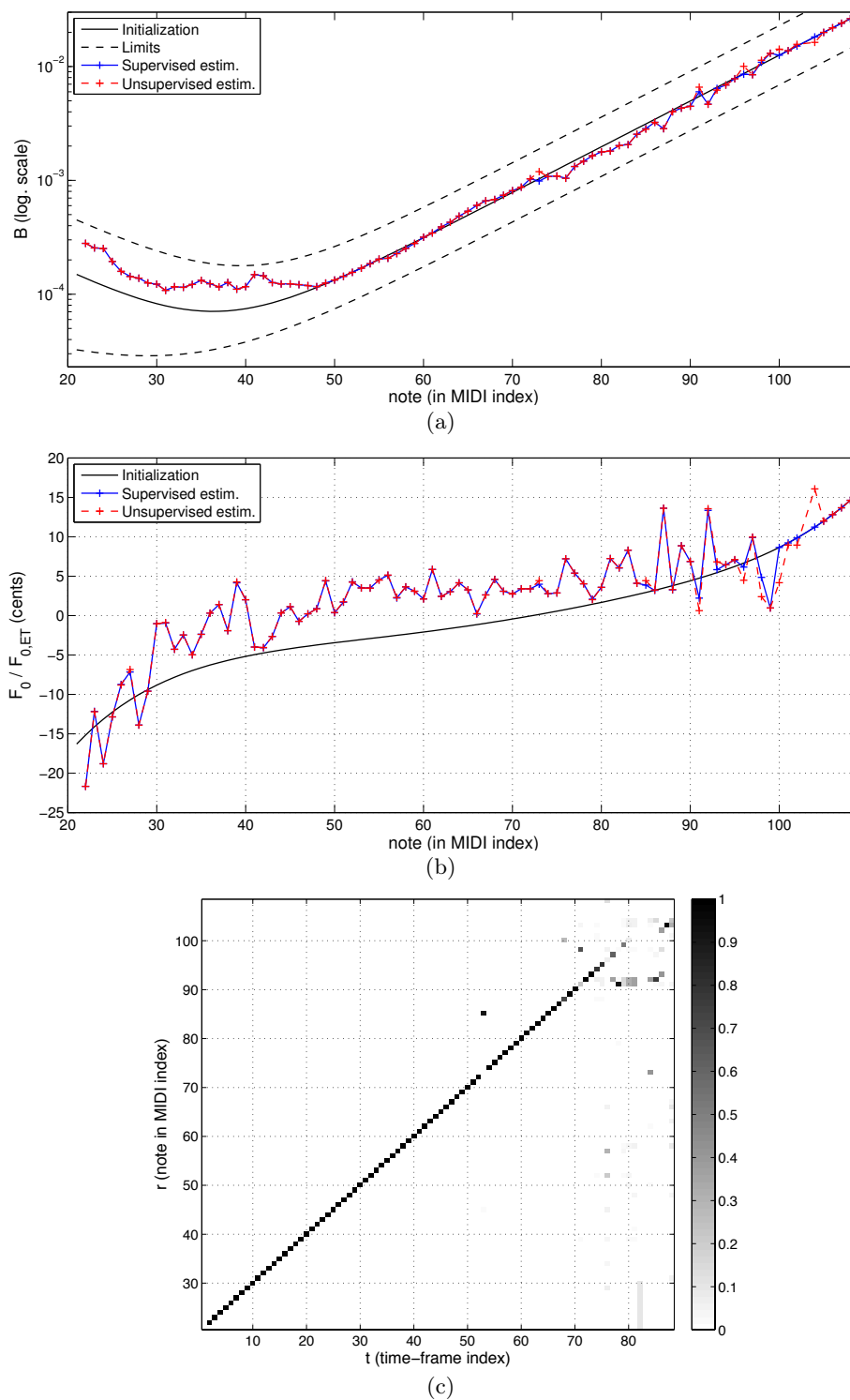
Figure 3.21: Analysis on the whole compass from isolated note recordings of Iowa piano. (a) B in log. scale and (b) F_0 as dev. from ET (in cents) along the whole compass. ( B , F_0 ) estimates are depicted as blue and red '+' markers, respectively for the supervised and the unsupervised cases. The initialization is plotted as gray lines and the limits for the estimation of B as gray dashed-lines. (c) \Omega returned by the unsupervised analysis.
