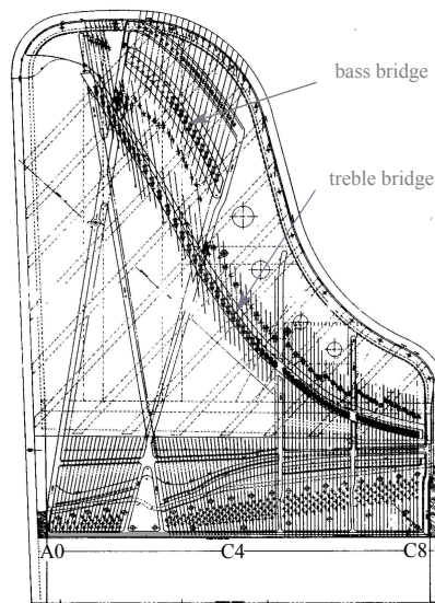
Figure 4.3: Grand piano string and bridge design. From [Conklin, Jr., 1996b].
