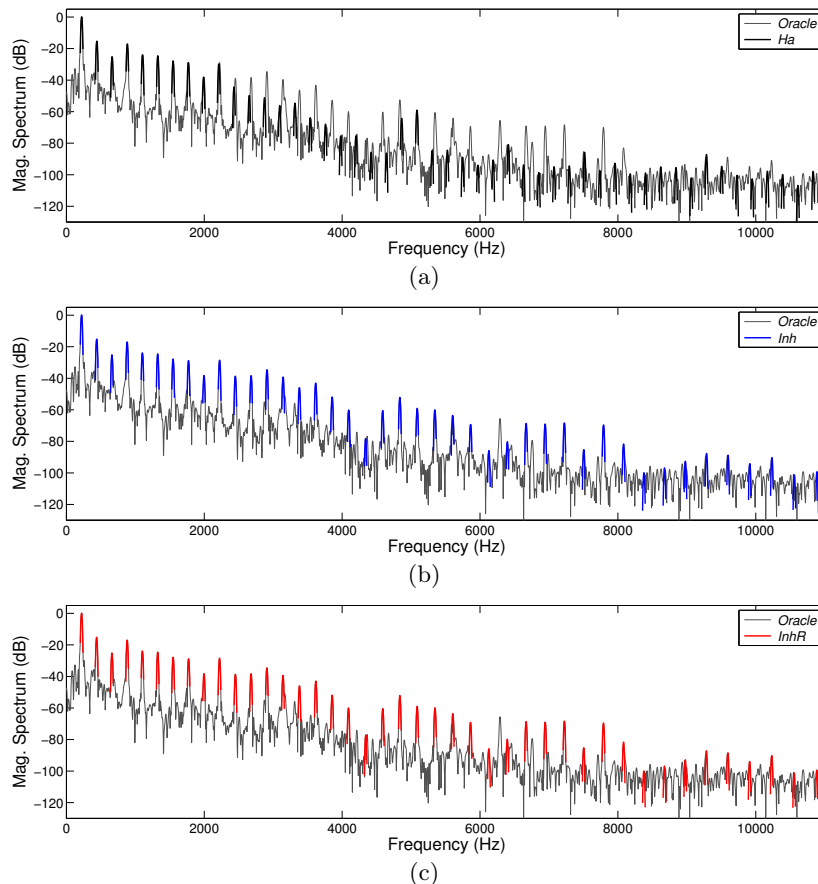
Figure 5.4: Spectrum of the note A3 (MAPS ENSTDkAM piano) for the dictionary of (a) Ha-NMF , (b) Inh-NMF , and (c) InhR-NMF . The original spectrum (in gray) is used for the dictionary of Oracle-NMF .
