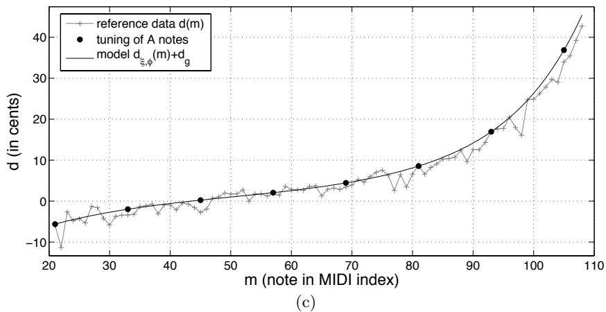
Figure 4.7: RWC2 grand piano. (a) Inharmonicity coefficient B , (b) octave type parameter \rho , (c) deviation from ET along the whole compass. The data are depicted as gray ‘+’ markers and the model as black lines.
