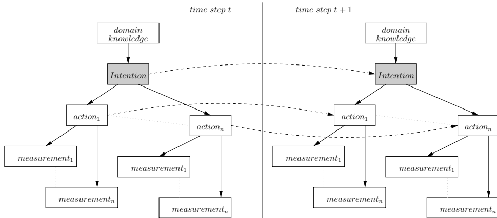
Figure 4.3: A generic DBN model for intention recognition.
