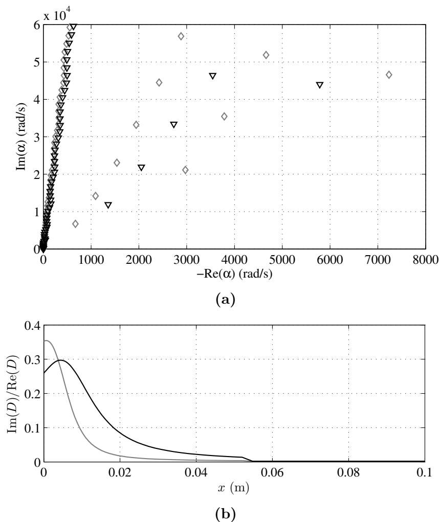
Figure 3.12: (a) Spectrum of the complex eigenvalues and (b) Equivalent loss factor for ABH with E_l=7 GPa ( \nabla , black) and E_l=1 GPa ( \diamond , grey).
