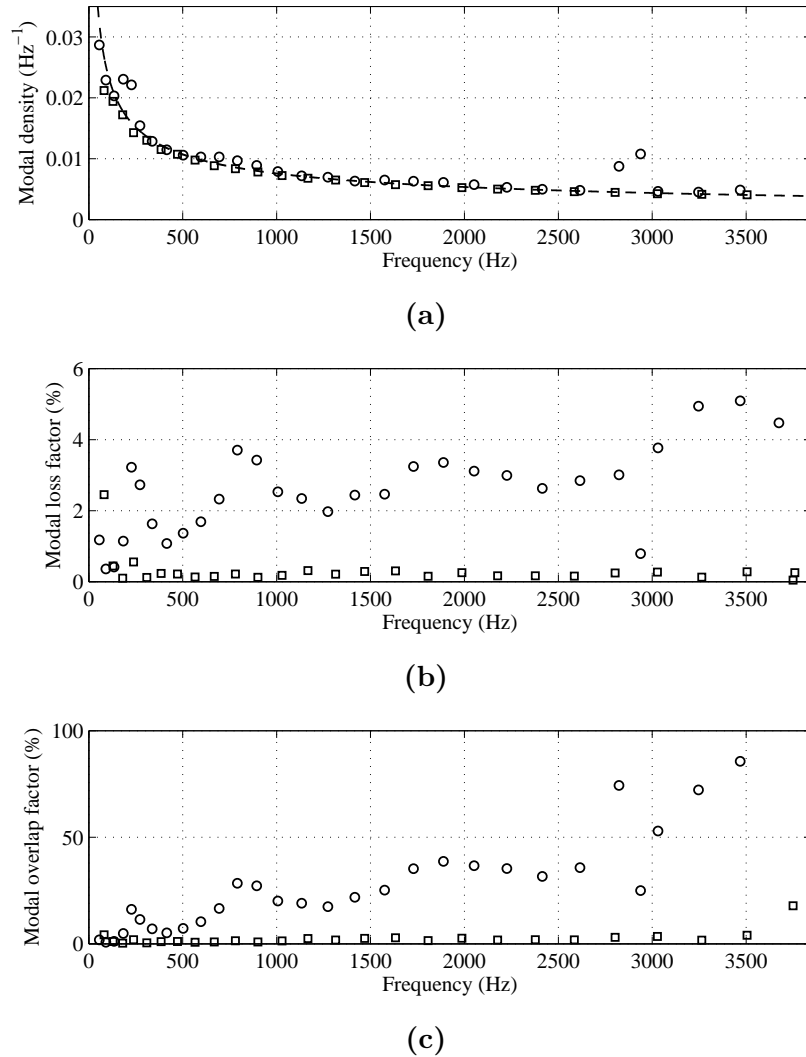
Figure 2.5: Comparison of experimental results between the aluminium reference beam (□) and the aluminium ABH beam (○): (a) Modal densities n and theoretical prediction for flexural waves in a uniform beam according to Eq. (2.4) (dashed line), (b) modal loss factors \eta , (c) Modal Overlap Factor MOF (published in [38]).
