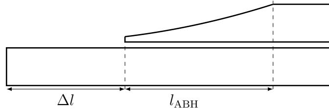
Figure 3.10: Scheme of the correction length induced by ABH.
