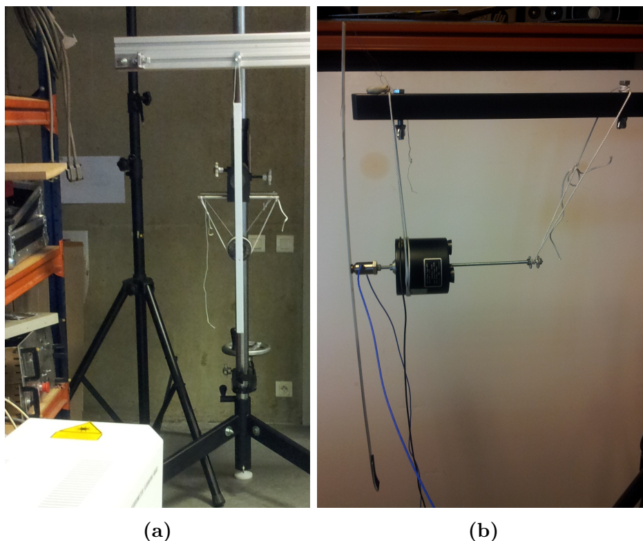
Figure 2.7: Picture of the experimental setup: (a) front view and (b) side view.
