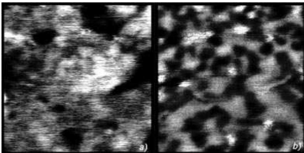
Fig. 4. (a) AFM topographic picture ( 256 \text{ nm} \times 256 \text{ nm} , contact mode, z scale: 2.5 \text{ nm} ) of the sample of Figure 3. (b) AFM friction picture ( 256 \text{ nm} \times 256 \text{ nm} , contact mode, z scale: 0.1 \text{ V} ) recorded at the same time. Ordered domains are lightly contrasted in the topographic picture, but appear as low friction areas in the friction picture.
