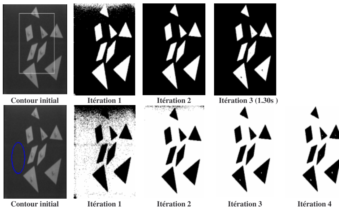
Figure 2.4: Segmentation de l'image Tangrame [256*256]
