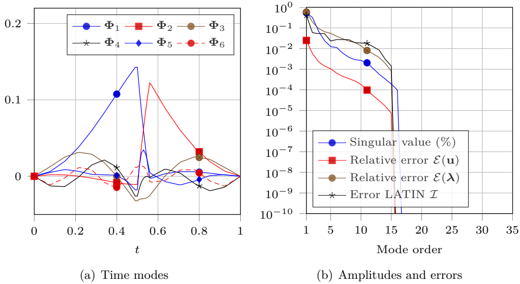
Figure 2.4 – SVD time modes of \mathbf{u}^* scaled by a corresponding factor 0.2\sqrt{\sigma_i} , singular value amplitudes and rebuilding errors according to the number of considered modes.
