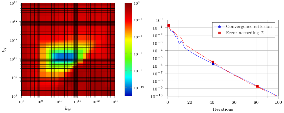
(a) Error reached according search direction parameters
