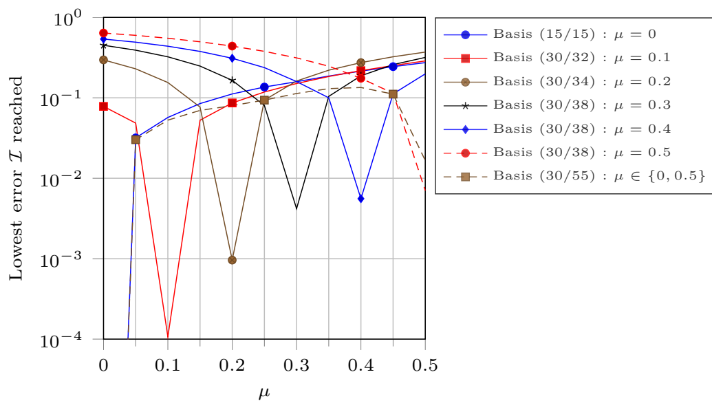
(b) LATIN-ROM with 30 space-time modes
