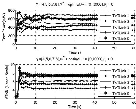
Figure 3.8: Autonomous adaptive transmission power execution
