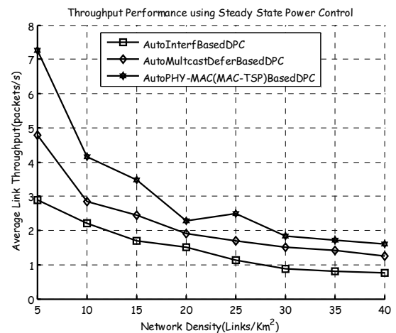
Figure 3.13: Average throughput performance at steady state power versus network density
