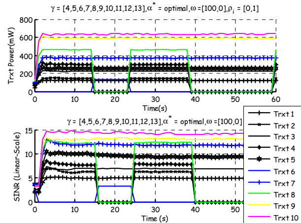
Figure 3.9: Autonomous dynamic power allocation incorporating power saving
