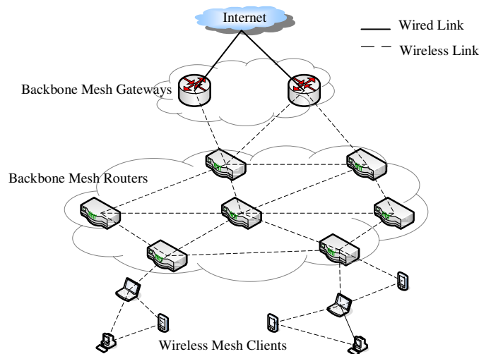
Figure 1.1: Hybrid Wireless Mesh Network architecture
