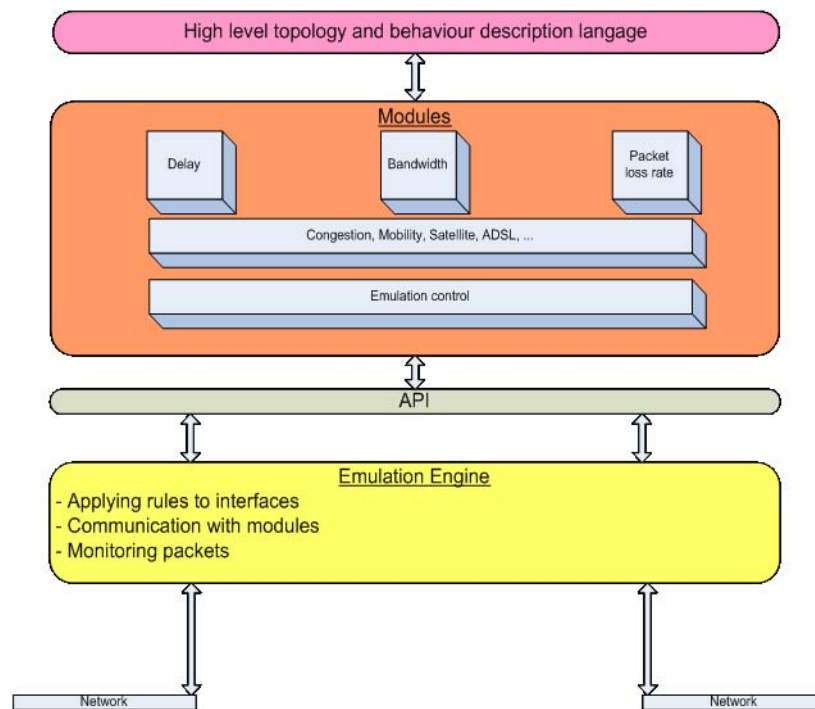
FIGURE 4.4 Architecture d'émulation active
