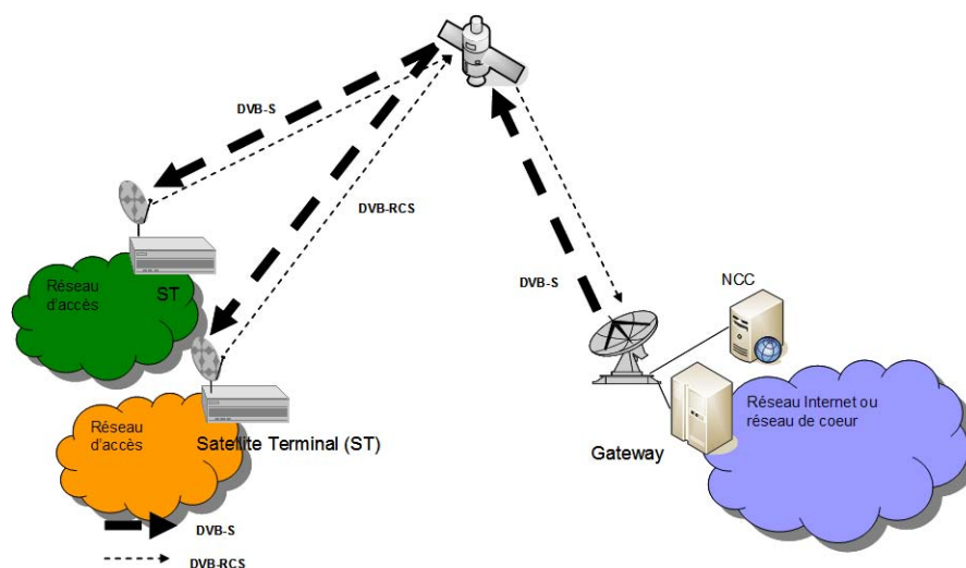
FIGURE 5.24 Architecture satellite étudiée
