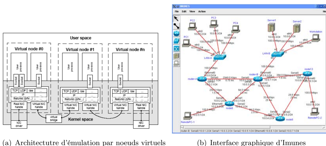
FIGURE 2.6 Emulation virtuelle
