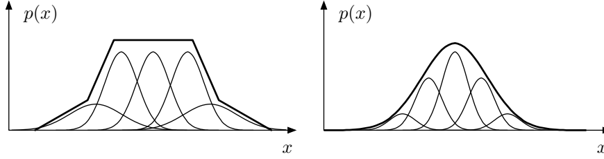
Figure 3.6: Gaussian sum approximations. Left: A non-Gaussian pdf . Right: A Gaussian pdf which is too large for the non-linearities. GSF will normally use both types of approach.
