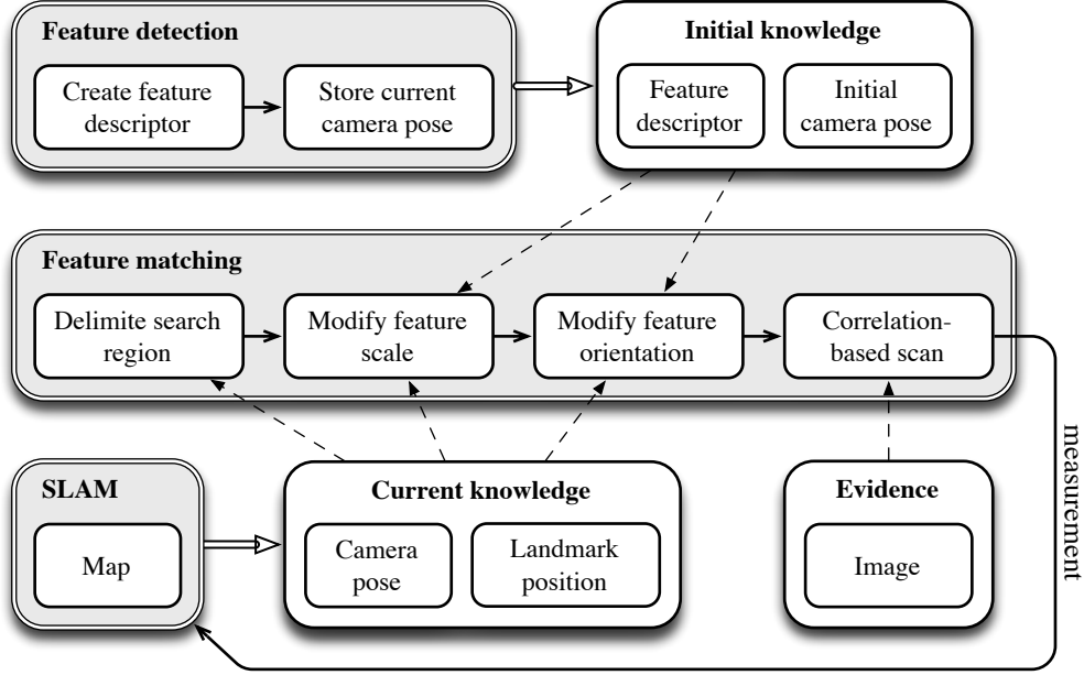
Figure 6.18: Active feature search (in the central gray thread) is guided by the available information (inside white boxes) which comes from the SLAM map and the feature detector, and by the current evidence provided by the perceived images.
