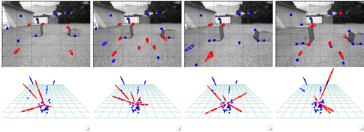
Figure 6.21: A portion of the reconstruction sequence at 5 frames (approx. 35cm) intervals. Image plane and 3D reconstruction are shown for frames 46, 51, 56 and 61.
