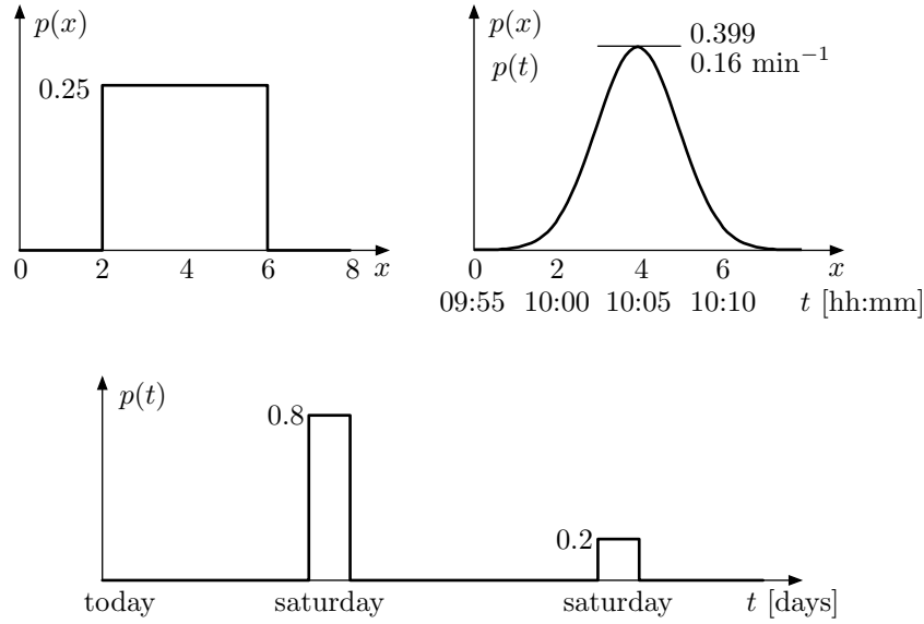
Figure 3.1: Three examples of pdf encoding different beliefs. Top left : Uniform distribution, ‘ X can be anything between 2 and 6’ or simply ‘ 2 \leq X \leq 6 ’. Top right : Gaussian distributions, p(x) says ‘ X is close to 4 with an uncertainty of \pm 1 ’; p(t) describes the knowledge ‘Tomorrow, ten o’clock’, something that is not likely to happen before 10:00, nor after 10:10, and expected around 10:05. Bottom : A bimodal distribution, ‘I think it’s this Saturday, but it could be next one.’
