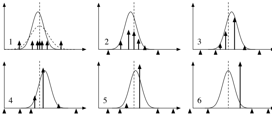
Figure 3.10: Particle degeneracy: a progressive degradation of the particle sum approximation. The true state is at the vertical dotted line, with an initial prior indicated by the dotted Gaussian in 1, which is approximated by the particle sum as shown. The noisy observations are represented by the solid Gaussian.
