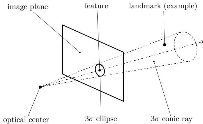
Figure 5.3: The conic ray extends to infinity.
