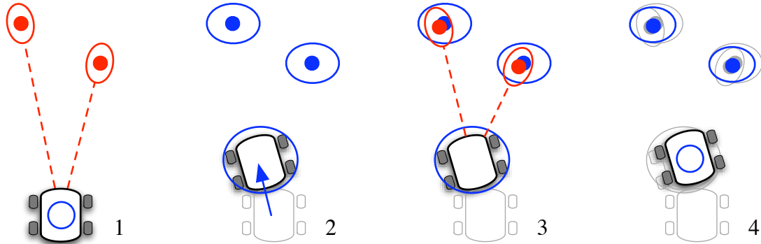
Figure 4.1: Typical SLAM operations during a complete filter loop. 1 : perception of new landmarks and their initialization in the map. 2 : Prediction of robot motion with associated increase of its position uncertainty. 3 : Observation of already mapped landmarks from an uncertain robot position. 4 : Correction of landmark positions and robot localization, with associated decrease of both robot and map uncertainties. Ellipses represent the uncertainty boundaries.
