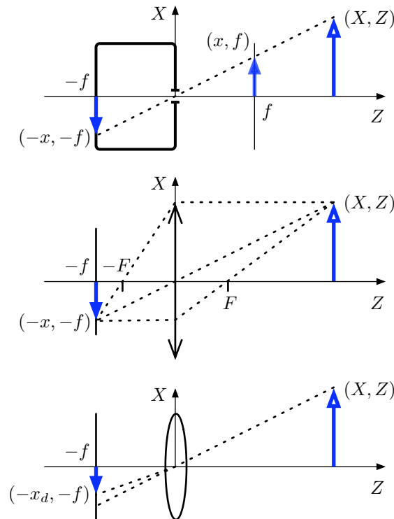
Figure 2.1: Modelling of a perspective camera. Light traveling in straight lines suffices to understand the Pin-Hole camera principle ( top ). An ideal, focused convergent lens accomplishes the same goal, with an enormous gain in luminosity ( center ). Distortion induced by real lenses must be taken into account ( bottom ).
