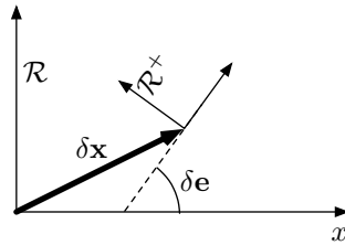
Figure 1.8: Odometry model with position and Euler increments.
