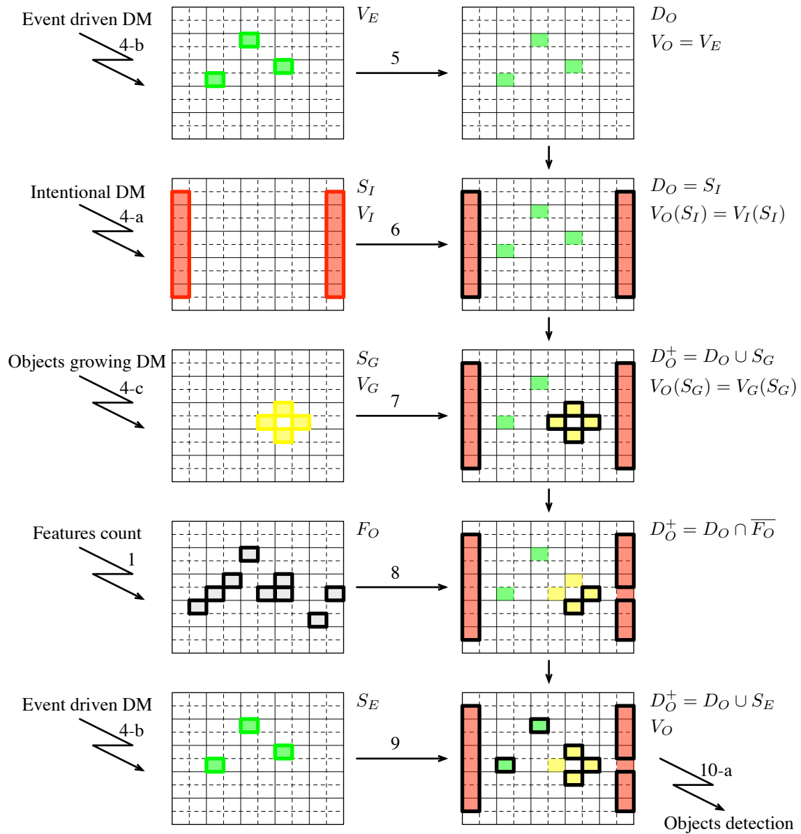
Figure 8.12: Priority-based Detection Selector algorithm -II-: Objects detection selector mechanism. The results of the different DM (left) sequentially update the output binary and velocity matrices D_O and V_O (right). A colored background indicates the nature of the velocity a-priori that has been set for that cell in V_O . Active cells in D_O are black-framed. Observe how the result (bottom-right) is a set of active cells with associated velocity a-prioris which respects the three imposed criterions.
