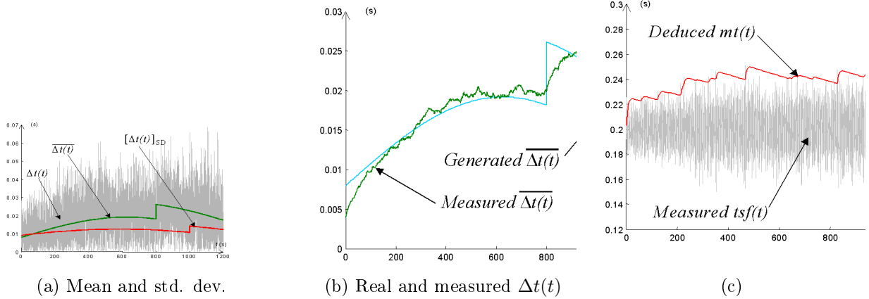
Figure 6: Generated delays
