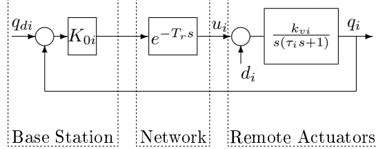
Figure 3: Transmission model
