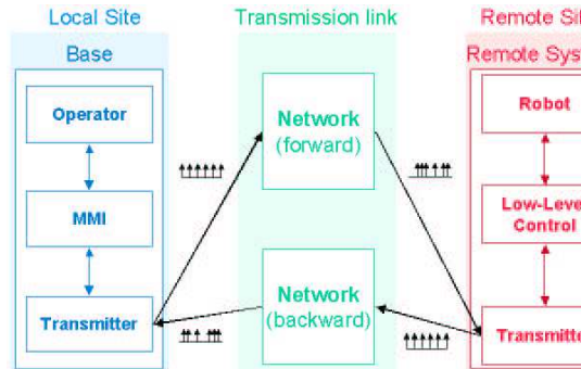
Figure 1: Teleoperation Architecture
