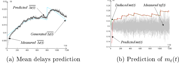
Figure 7: Delays prediction
