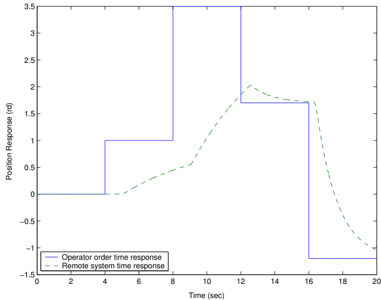
Figure 11: Effects of the HOSM on q_1(t)
