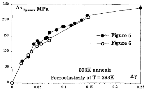
Figure 11 : \Delta\tau_{hysmax}(\Delta\gamma) in ferroelasticity
