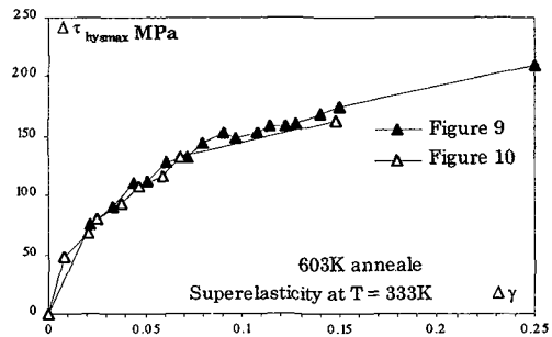
Figure 12 : \Delta\tau_{hysmax}(\Delta\gamma) in superelasticity
