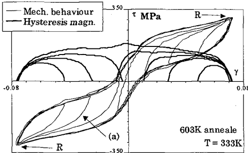
Figure 7 : Subloops and hysteresis magnitude with increasing values of \Delta\gamma in superelasticity, start point at \gamma = \gamma_{\text{max}} .
