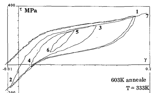
Figure 10 : Discrete memory concept in superelasticity
