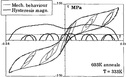
Figure 5 : Subloops and hysteresis magnitude with \Delta\gamma = 1.5\% in superelasticity.
