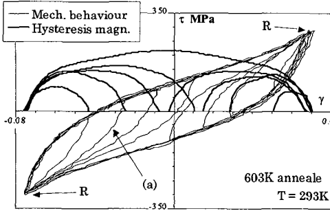
Figure 3 : Subloops and hysteresis magnitude with increasing values of \Delta\gamma in ferroelasticity, start point at \gamma = \gamma_{\text{max}} .
