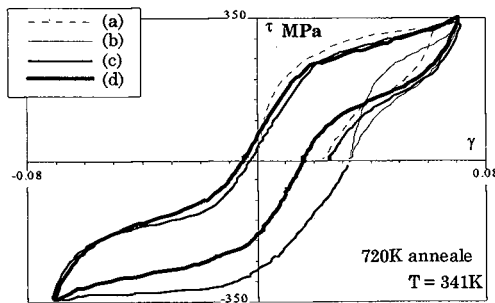
Figure 1 : Influence of the loading path on the hysteresis study
