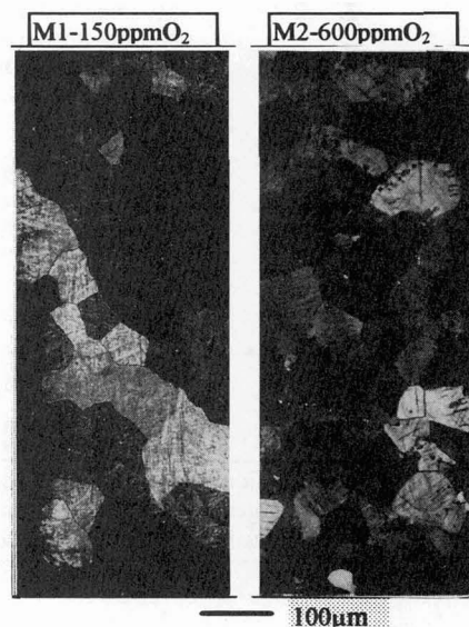
Figure 4: Microstructure of hot rolled samples (annealed 24h at 900^{\circ}C containing various amount of oxygen
