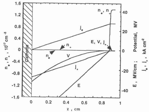
Fig. 5 Derived cathode sheath properties for S=2 \times 10^{23} [3].
