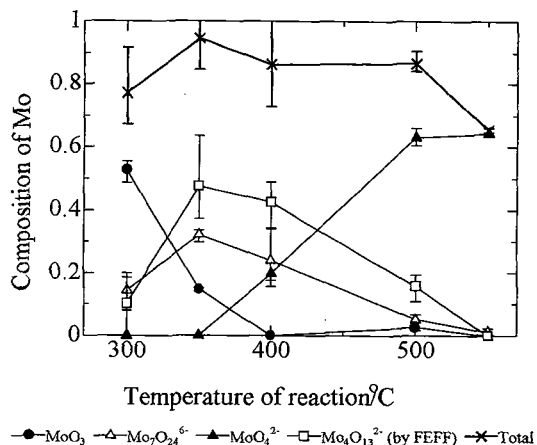
Fig.3 Composition of Mo species in samples obtained from Mo precursors by quenching at various temperatures obtained from EXAFS data by fitting using reference data.
