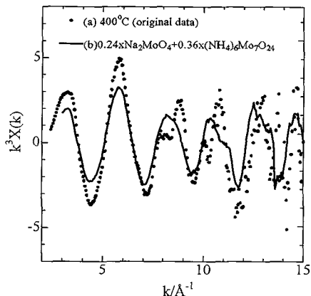
Fig.2. Fitting of EXAFS data in k -space using reference data.
