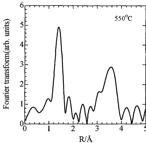
Fig.4 Fourier transform of residual k^3X(k) after subtraction of the fitting result for Mo K-edge EXAFS of the sample at 550 °C.
