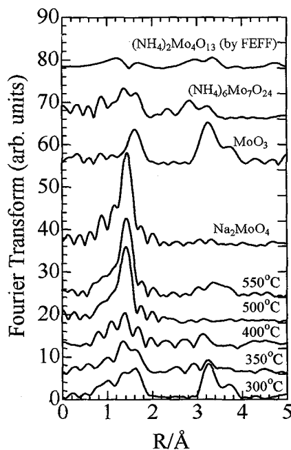
Fig.1 Fourier transforms of Mo K-edge EXAFS for samples obtained from Mo precursors by quenching at various temperatures.
