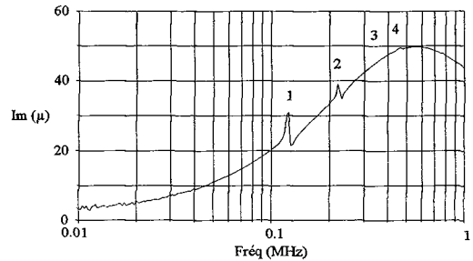
Fig 2 : Experimental imaginary permeability
