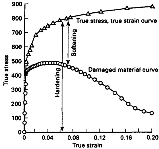
Figure 1 : Stress-strain curve accounting for damage
