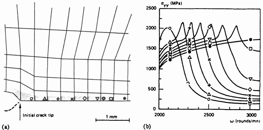
Figure 2 : a) Stable crack growth modelling (damaged zone in grey), and b) evolution of opening stress at the crack tip (the symbols correspond to the location in a))
