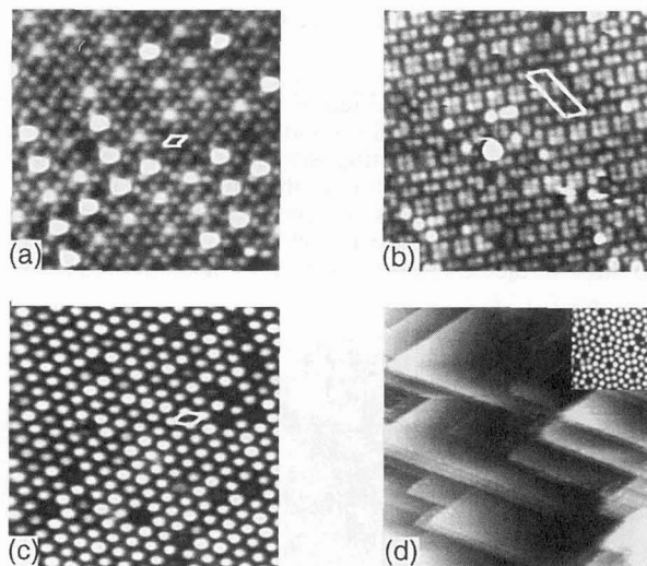
Figure 2: Sequence of STM images of the 6H-SiC(0001) surface, showing the Si rich structures in the order of increasing Si concentration: (a) The (2\times 2) reconstruction ( 120\text{ \AA}\times 120\text{ \AA} ); (b) The (2\sqrt{3}\times 6\sqrt{3}) reconstruction ( 118\text{ \AA}\times 118\text{ \AA} ); (c) The (3\times 3) reconstruction ( 160\text{ \AA}\times 160\text{ \AA} ); (d) The (7\times 7) reconstruction ( 1200\text{ \AA}\times 1200\text{ \AA} ). The insert shows an empty-state image (+2V) of the (7\times 7) structure.
