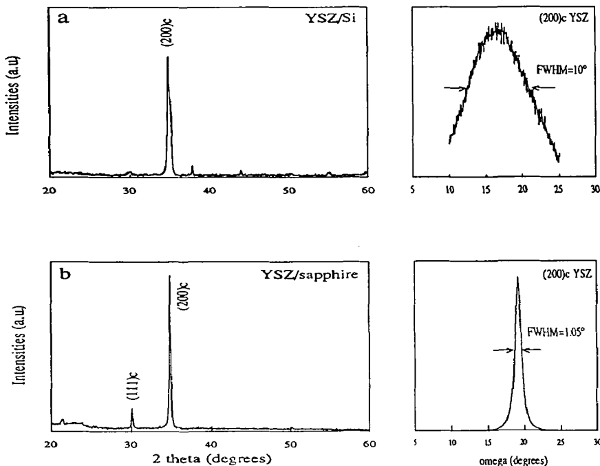
Figure.1: XRD pattern of YSZ deposited on (a) silicon at 750°C and (b) on sapphire (1-102) at 820°C. Rocking scans through (200) reflection of YSZ film deposited on silicon and on sapphire are also shown.
