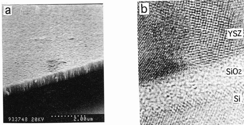
Figure.3: (a) SEM cross-section micrograph of an YSZ layer deposited on silicon (b) TEM micrograph of the \text{SiO}_2 interlayer observed between silicon and YSZ.
