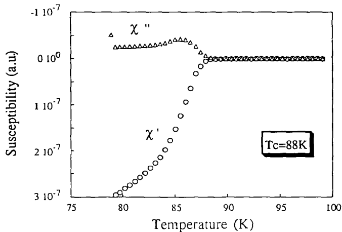
Figure.8 : A C-susceptibility curve vs temperature for a multilayer YBCO/YSZ/sapphire. \chi' and \chi'' are the real and imaginary parts of the AC-susceptibility.
