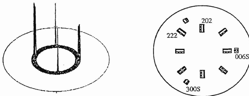
figure.2: (202)-YSZ reflection pole figure (on the left). A combined (202) and (222)-YSZ reflections and (006) and (300)- sapphire reflection pole figures (on the right side).
