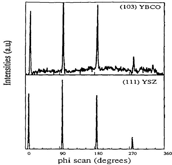
Figure.7: phi-scan patterns of (103)-YBCO and (111)-YSZ reflections.
