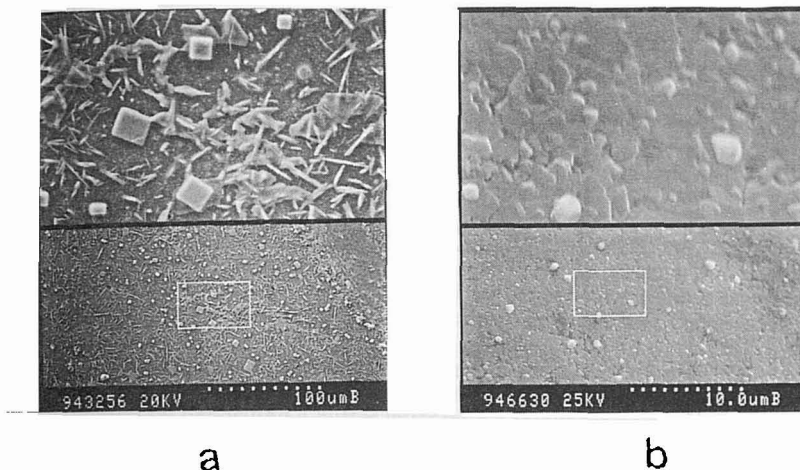
Figure.5: SEM micrograph of the surface of an YBCO layer grown on YSZ/Si by MOCVD at (a) 910°C and (b) 845°C.
