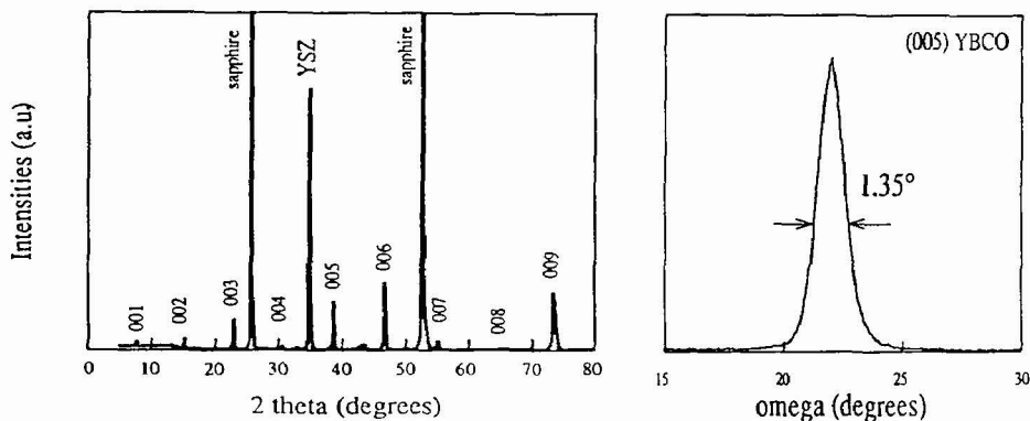
Figure.6: XRD pattern of YBCO deposited on sapphire with an (100) epitaxial YSZ buffer layer. Figure on the right shows the rocking scan across the (005) YBCO reflection.
