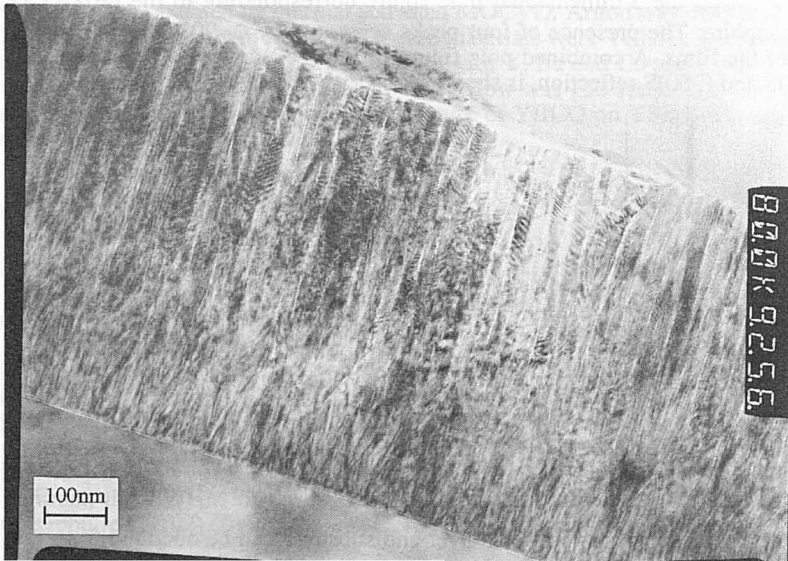
Figure.4: TEM micrography of a YSZ buffer layer obtained on sapphire at 820°C.
