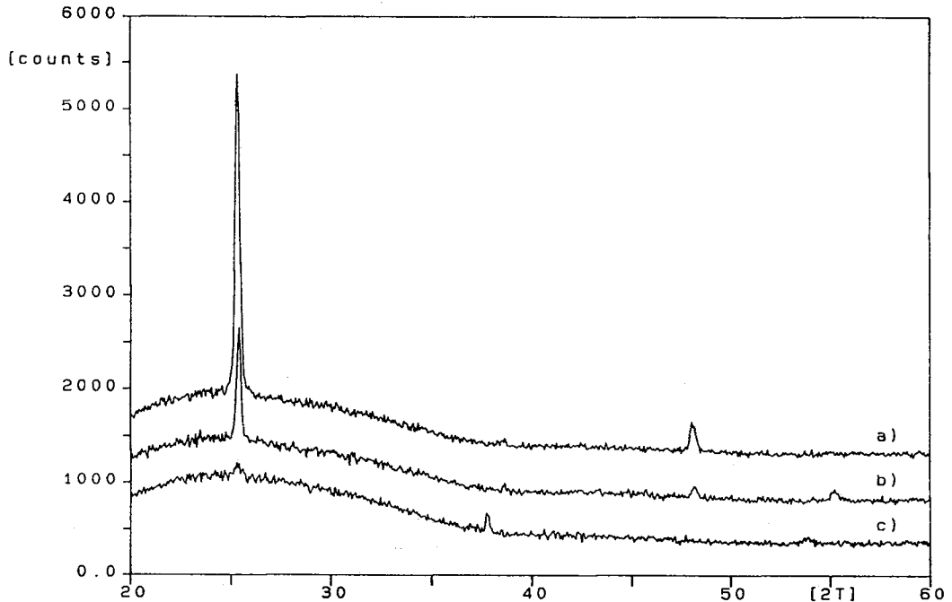
Figure 3: XRD patterns of 120 nm thick \text{TiO}_2 films grown on soda lime glass substrates from (a) titanium tetraisopropoxide at 325 °C, (b) titanium tetraethoxide at 250 °C and (c) \text{TiCl}_4 at 500 °C. In all the cases the other precursor was water.
