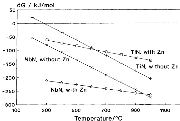
Figure 2: Gibbs energy vs. temperature for the growth reactions of TiN and NbN with and without Zn [44].
