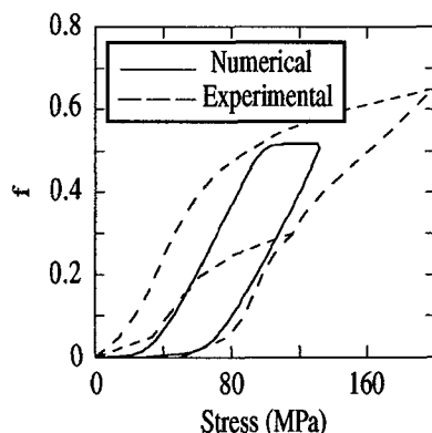
Figure 2: Kinetics of a stress-induced transformation. Comparison between experiment results [14] and self-consistent determination for tensile test at T = -80^{\circ}\text{C} ( M_s = -97^{\circ}\text{C} A_f = -91^{\circ}\text{C} ).
