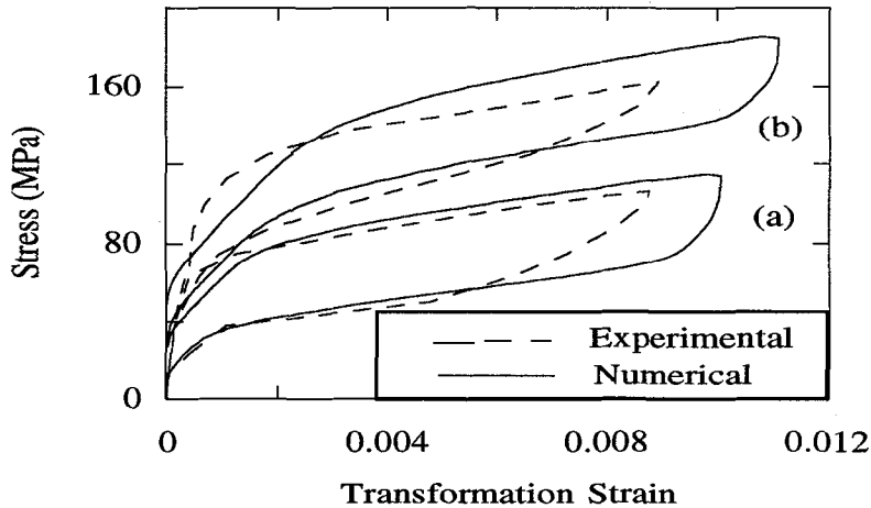
Figure 1: Influence of the temperature on the superelastic behavior. Comparison between experiment results [14] and self-consistent determination ( M_s = -97^\circ\text{C} , A_f = -91^\circ\text{C} , T_a = -80^\circ\text{C} , T_b = -70^\circ\text{C} ).
