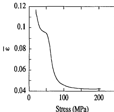
Figure 3: Evolution of the mean Transformation Strain for an uniaxial tensile test experiment.
