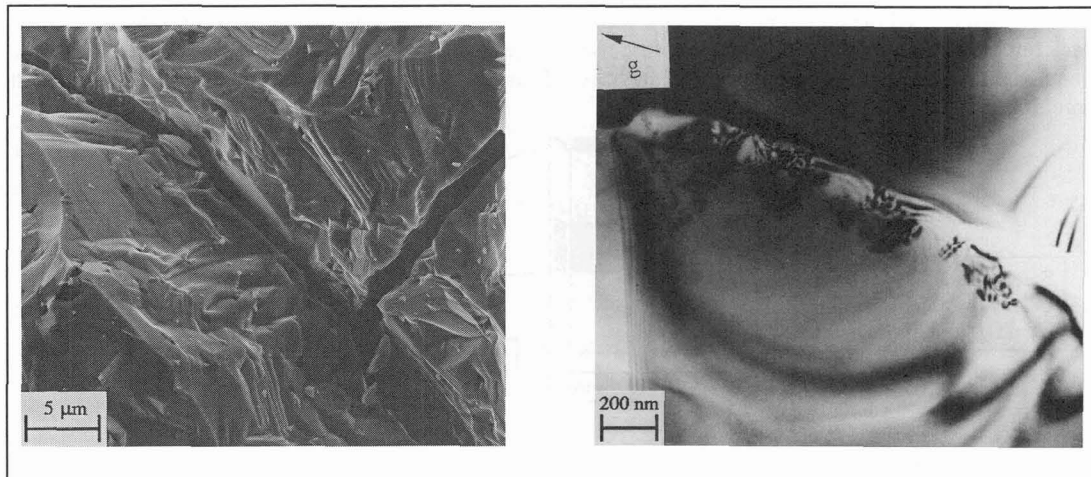
Figure 2 : Scanning Electronic Microscopy Transgranular propagation of the crack
